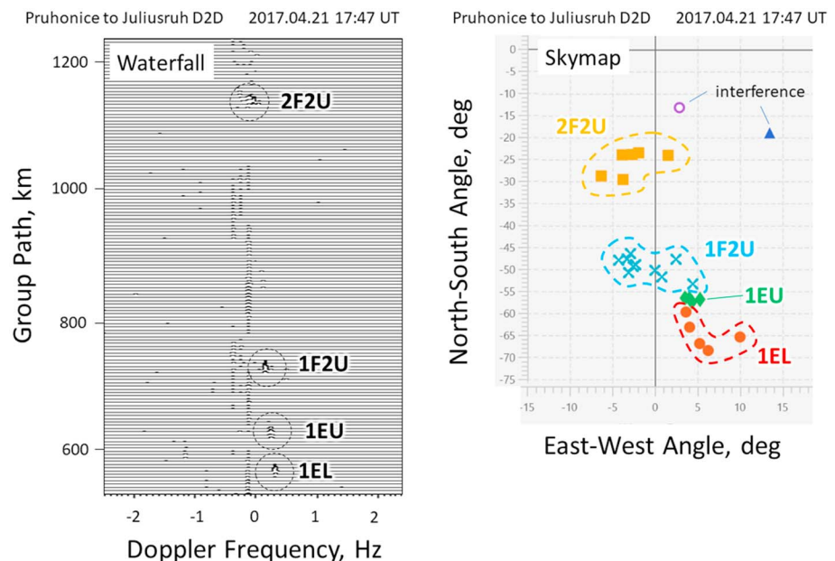
Figure 4. Digisonde-to-Digisonde (D2D) measurements for northern Pruhonicne to Juliusruh link, f = 5.05 MHz; Doppler waterfall and skymap.
