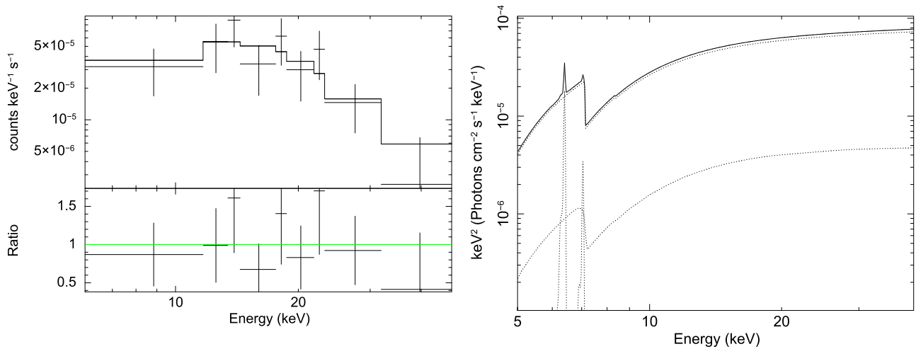
Figure 6. Left panel: combined NuSTAR FPMA and FPMB spectrum of WISE J1036+0449 fitted with the MYTORUS model (assuming \Gamma = 1.9 ; see Section 4). The bottom panel shows the ratio between the data and the model. Right panel: spectrum of the MYTORUS model with the parameters fixed to those obtained by fitting the combined NuSTAR FPMA and FPMB spectrum. The dotted lines represent the primary X-ray emission (upper part of the figure), the scattered component (lower part), and the fluorescent lines. In both plots, the energies are in the rest frame of the source.
