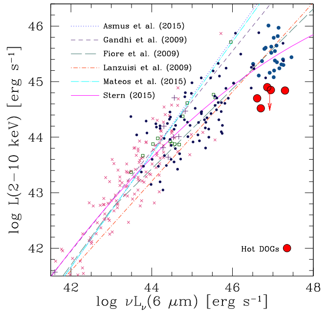
Figure 8. Rest-frame 6\ \mu\text{m} luminosity vs. intrinsic rest-frame 2–10 keV luminosity for several samples of AGNs: Hot DOGs from this work (big red circles; the red arrow represents the upper limit for WISE J2207+1939), broad-lined AGNs from the SEXSI survey (Eckart et al. 2010; open green squares), luminous quasars from Just et al. (2007; large solid blue circles), Compton-thin AGNs observed by NuSTAR (Alexander et al. 2013; Del Moro et al. 2014; purple crosses), quasars from SDSS DR5 (Young et al. 2009; small blue dots), and local Seyfert galaxies (Gandhi et al. 2009; Asmus et al. 2015; red crosses). The lines illustrate five L_{6\ \mu\text{m}}-L_{2-10\ \text{keV}} relations (see Section 5.2 for details). The mid-IR luminosities of Asmus et al. (2015) were obtained at 12\ \mu\text{m} . The figure shows that hot DOGs are significantly weaker in the X-ray band than unobscured quasars in the same 6\ \mu\text{m} luminosity range.
