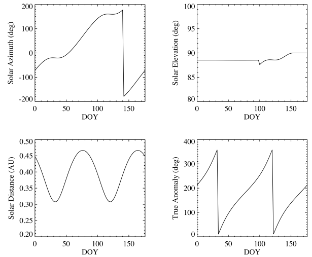
Figure 5. Average illumination conditions above Prokofiev and Kandinsky craters and Mercury’s orbital parameters for one hermean solar day. The illumination rendering shown in the previous Fig. 4 at \text{TA}=200^\circ corresponds to \text{DOY}=84 .
