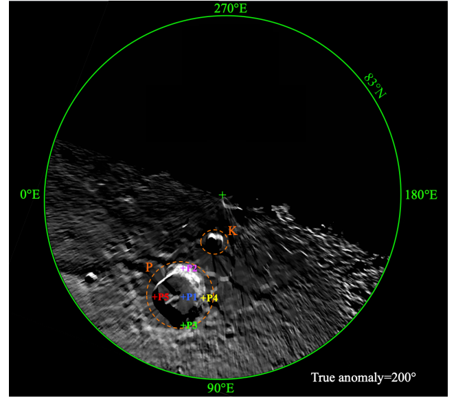
Figure 4. Illumination rendering on the north polar regions for \text{TA}=200^\circ . The full simulation covering an entire solar day is available as a supplemental online material. Locations P1-5 are shown for Prokofiev (similar positions for Kandinsky are shown in Fig. 9) at larger scale.
