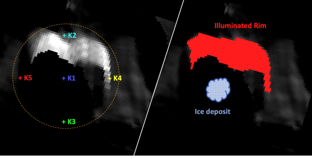
Figure 9. Simulated illumination conditions, or \cos(i) , occurring on Kandinsky crater at TA=200^\circ (left panel). The area of the sun illuminated rim (in red, departing from point K2) and the location of the putative water ice deposit (blue dots, corresponding to location K1) on the unilluminated crater floor are shown on the right panel.
