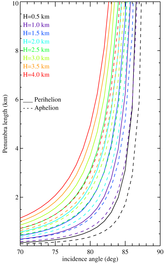
Figure 3. Penumbra length cast by the Sun at at perihelion (solid line) and aphelion (dashed line) from a crater’s rim of variable height between 0.5 to 4 km placed at latitude 80^\circ .
