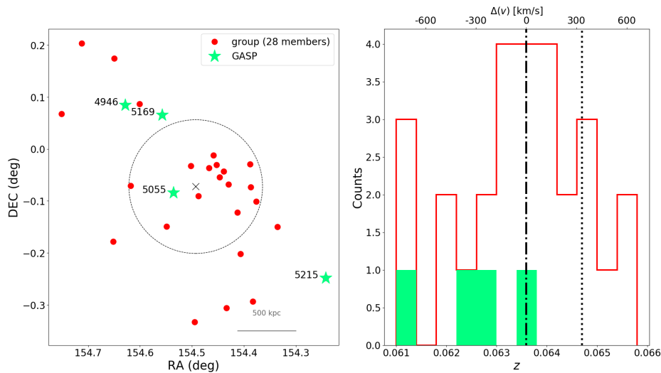
Figure 2. Left: Position in the sky of the group and of its members. The galaxies that will be further analysed in the paper are highlighted with the green stars. The black dashed circle indicates the virial radius of the group. The scale in the bottom right corner shows 500 kpc at the redshift of the group. Right: Redshift distribution of the galaxies in the group. The GASP galaxies are highlighted in green. Dotted line is the group redshift given in Tempel et al. (2014b), dash-dotted line is the redshift adopted in this work. The upper axis shows the velocity difference with respect to the group redshift.
