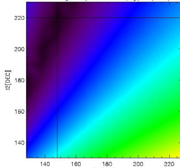
optimal at [I1,I2]= [148,220] CPV PSW Tuning LFI #27 M1- dV2
