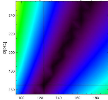
optimal at [I1,I2]= [124,165] CPV PSW Tuning LFI #27 M2- dV2
