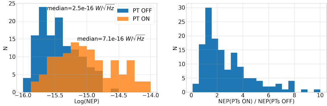
Figure 27. Left: Histogram of NEP measured between 1 Hz and 2 Hz in the transition ( V_{\text{bias}} = 1.5\text{V} ) with PTs ON and OFF. The response is assumed to be given by 1/V_{\text{TES}} . The total number of TES are 130 and 120 respectively. Right: Histogram of the ratio of NEP with PTs ON and NEP with PT OFF. The total number of TES is 143.
