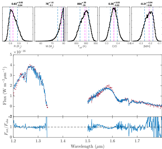
Figure 12. Top: Posterior distributions of derived quantities for the retrieval of HD 19467 B. The posteriors are shown for the brown dwarf radius R , its mass M , effective temperature T_{eff} , the C/O ratio, and the overall metallicity [M/H] . Bottom: Posterior spectra and residuals. The solid lines refer to the median of all posterior spectra. The shaded areas signify the 3\sigma confidence intervals of the spectra. The measured spectrum is indicated by the red data points.
