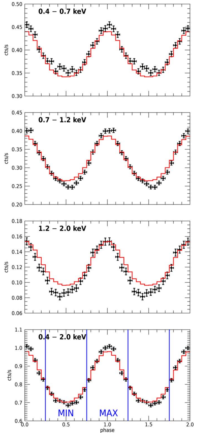
Figure 2. Background-subtracted pulse profiles in three energy ranges (0.4–0.7 keV, upper panel; 0.7–1.2 keV, middle panel; and 1.2–2 keV, lower panel), and in the total energy range 0.4–2 keV (bottom panel). The red lines represent the pulse profiles computed with our best-fit spectral model (see Section 2.2). The blue vertical lines show the phase intervals used to extract the spectra of the maximum and the minimum.
