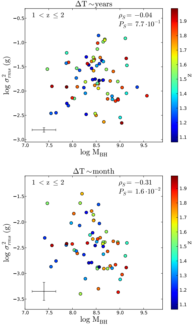
Fig. 4. Excess variance ( g_{P1} band) measured on timescales of years ( top ) and months ( bottom ) versus M_{\text{BH}} in units of M_{\odot} for the 1z2_MBH sample. Spearman's r and the respective p -value are reported in each sub-panel. The redshift is given as a color bar. The black error bars correspond to the average values.
