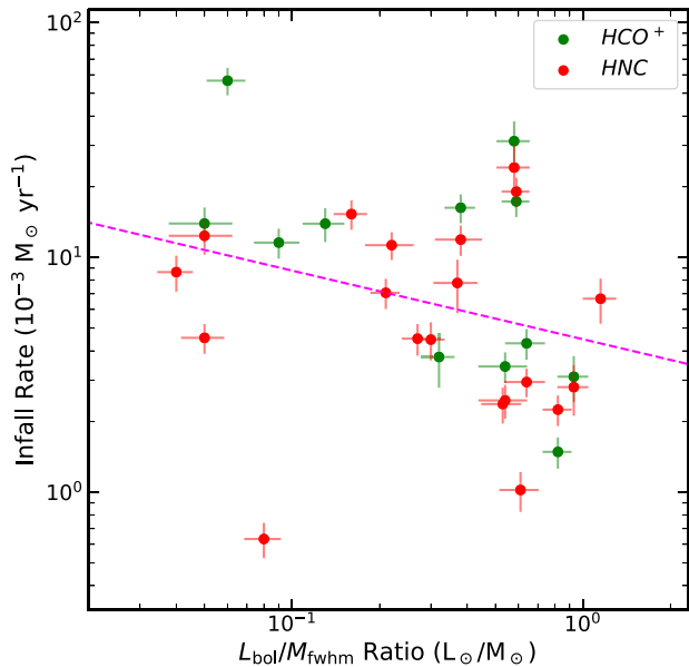
Figure 7. Mass infall rates as a function of the L/M ratio. The values determined from the two transition are shown in different colours, and the dashed line shows the results of a linear least squares fit to the log values of both parameters (slope = -0.29 \pm 0.18 , intercept = 0.65 \pm 0.12 ).
