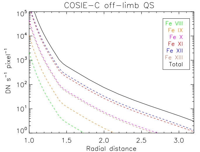
Figure 7. Estimated total count rates (per pixel) in the COSIE-C broadband, as a function of the radial distance, for the quiet Sun, using the UVCS model. The total rates are shown, as well as those produced by the main ions.
