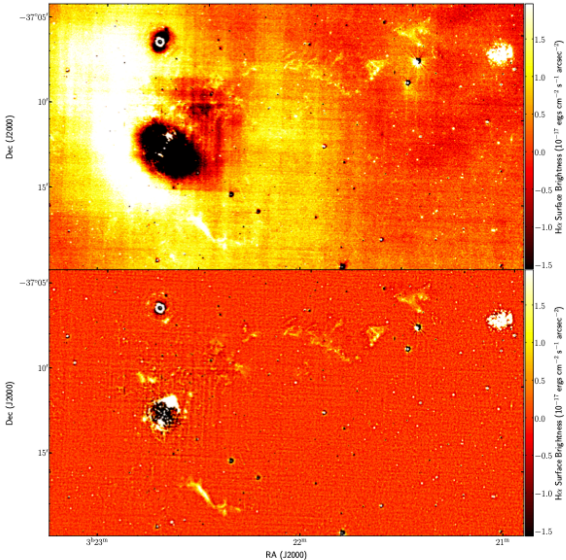
Fig. A.1. Comparison of the original and filtered H \alpha images. Top image: H \alpha image after the standard data reduction process. Bottom image: H \alpha image we present in our work that iteratively modelled and subtracted (described in Sect. 3.2) the background of the original image. Both images are presented on the same scale. The original image is clearly dominated by over- and under-subtracted artefacts, while the new image has a smooth and uniform background, which retains the majority of the real H \alpha emission. Some diffuse H \alpha emission is lost in this process, however, the new image is a significant improvement that shows the underlying structure of the giant H \alpha filaments in the IGM.
