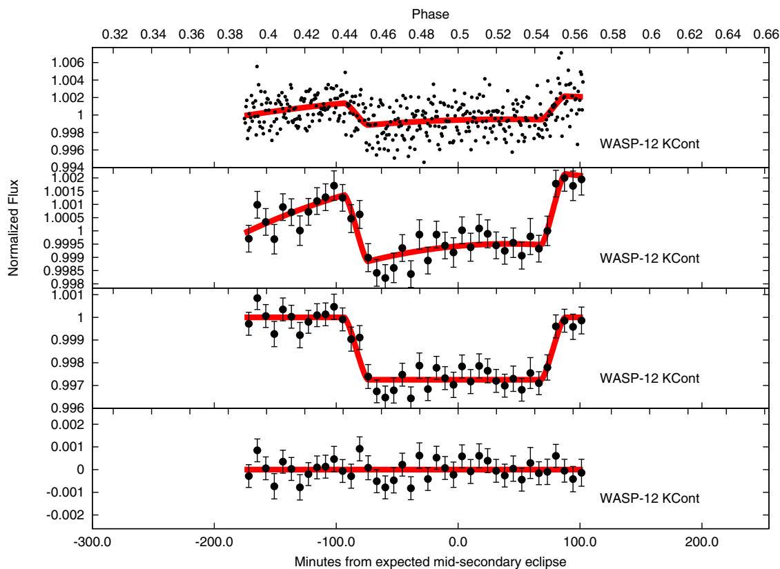
Figure 6. CFHT/WIRCam photometry of the secondary eclipse of WASP-12b observed in the K_{CONT} band on 2012 January 19. The format is otherwise identical to Figure 2.
