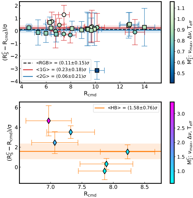
Fig. E.1. Difference between the photometric ( R_{\text{CMD}} ) and the asteroseismic ( R_{\text{S}} ) radii for our RGB (top) and rHB (bottom) stars. The black dashed line in the upper panel is the average dispersion of the entire sample, while the coloured lines represent the average value of each population with their 1\sigma intervals as the shaded areas.
