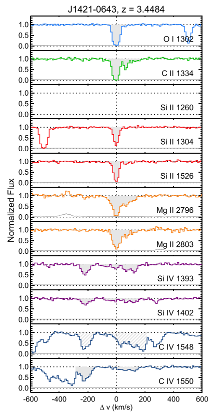
Figure 15. Stacked velocity plot for the z = 3.4484 system toward J1421-0643. Lines and shading are as described in Figure 11.
