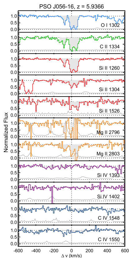
Figure 71. Stacked velocity plot for the z = 5.9366 system toward PSO J056–16. Lines and shading are as described in Figure 11.
