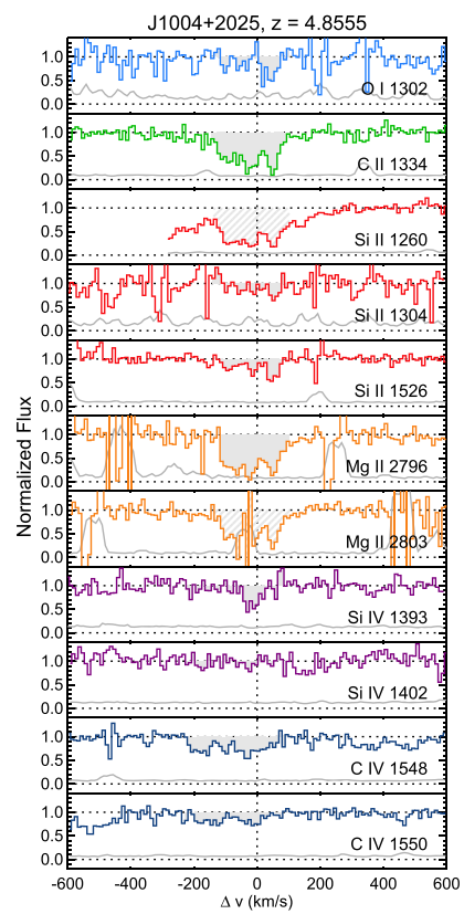
Figure 47. Stacked velocity plot for the z = 4.8555 system toward J1004+2025. Lines and shading are as described in Figure 11. See notes on this system in Appendix B.
