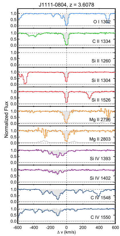
Figure 19. Stacked velocity plot for the z = 3.6078 system toward J1111-0804. Lines and shading are as described in Figure 11.
