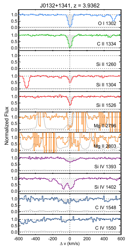
Figure 31. Stacked velocity plot for the z = 3.9362 system toward J0132+1341. Lines and shading are as described in Figure 11.
