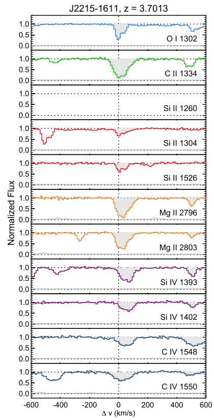
Figure 23. Stacked velocity plot for the z = 3.7013 system toward J2215–1611. Lines and shading are as described in Figure 11. See notes on this system in Appendix B.
