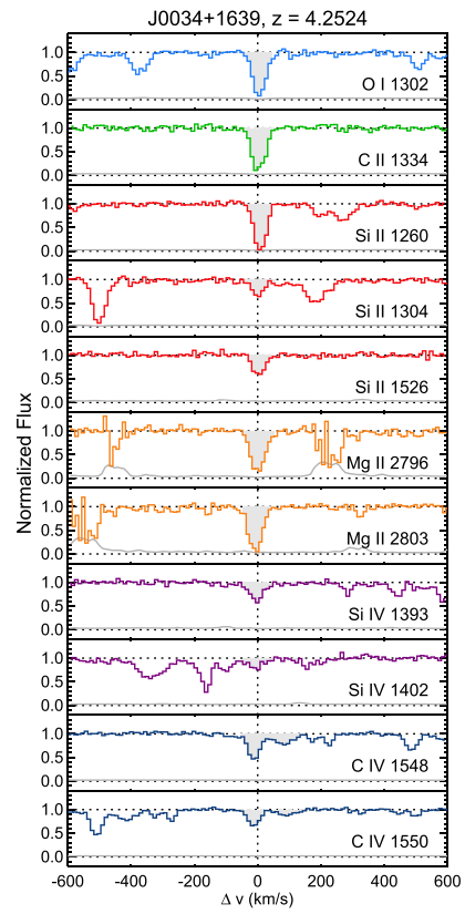
Figure 43. Stacked velocity plot for the z = 4.2524 system toward J0034+1639. Lines and shading are as described in Figure 11.
