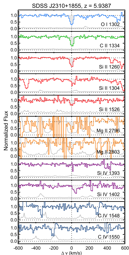
Figure 72. Stacked velocity plot for the z = 5.9387 system toward SDSS J2310+1855. Lines and shading are as described in Figure 11.
