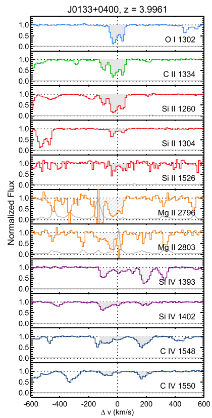
Figure 35. Stacked velocity plot for the z = 3.9961 system toward J0133+0400. Lines and shading are as described in Figure 11.
