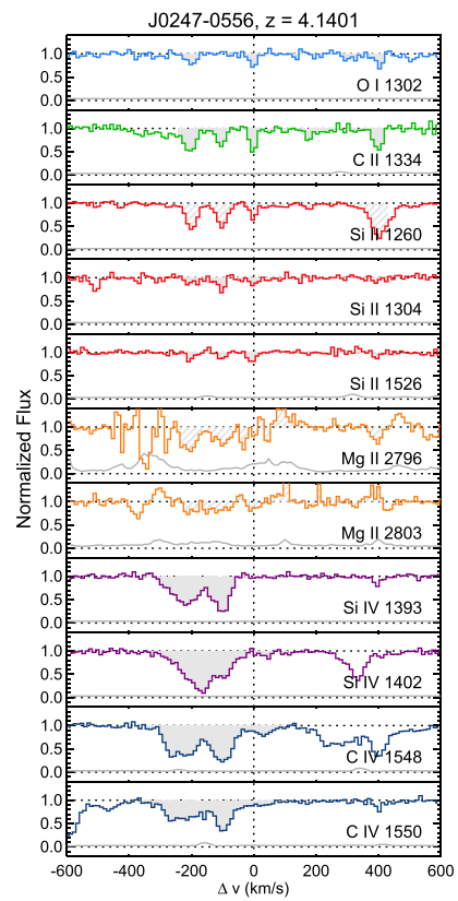
Figure 39. Stacked velocity plot for the z = 4.1401 system toward J0247 -0556. Lines and shading are as described in Figure 11. See notes on this system in Appendix B.
