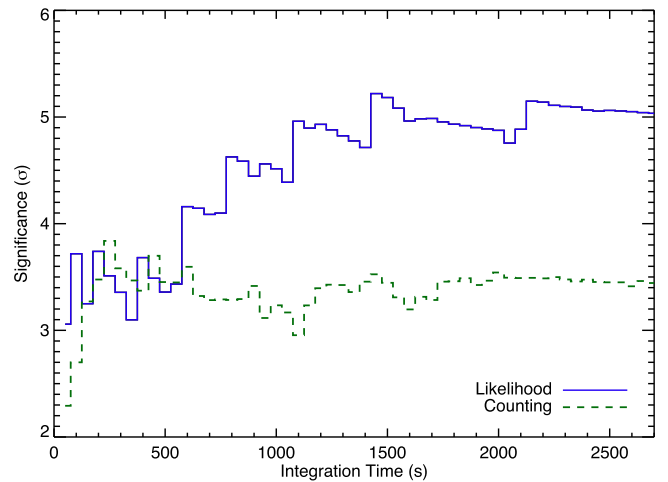
Figure 10. Comparison of the significance of the detected signal as a function of integration time, covering an energy range from 300 MeV to 30 GeV for a 10^\circ ROI selection, for both the counting and likelihood techniques.
