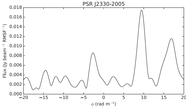
Figure 17. Faraday dispersion function for PSR J2330–2005 from epoch 1 after correcting for the effects of ionospheric Faraday rotation. RM = +9.6 rad m -2 . Noise is 1 mJy beam -1 RMSF -1 rms.
