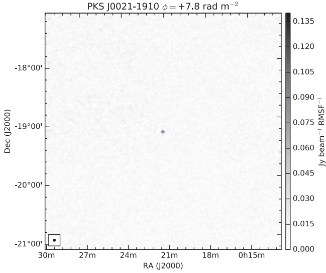
Figure 14. Cut-out showing the polarized source PKS J0021-1910. The synthesized beam is 2.2' \times 2.4' FWHM with a position angle of -47^\circ .
