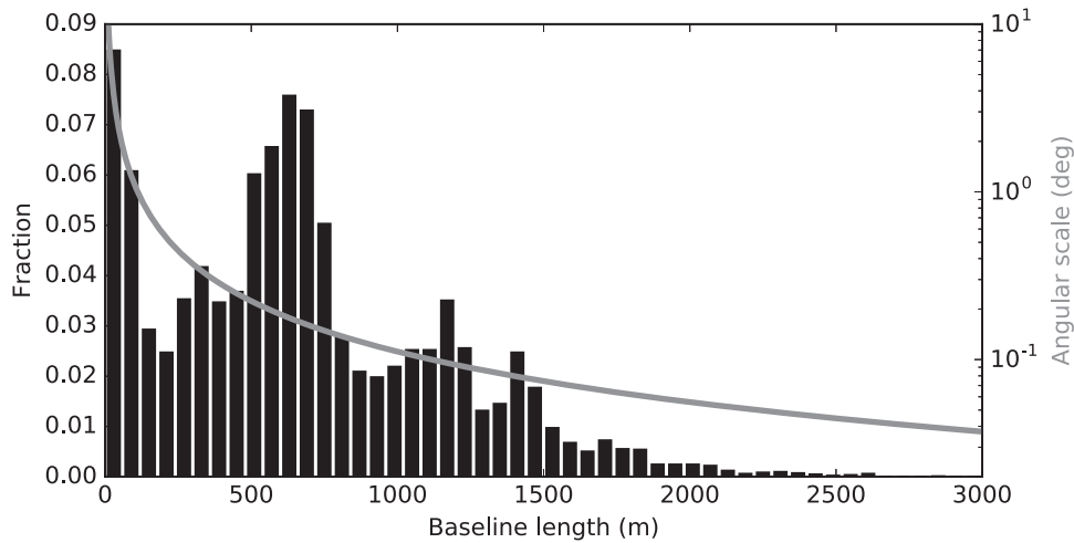
Figure 18. Snapshot imaging baseline distribution for MWA 128T when observing at zenith ( \delta = -26.7^\circ ). The gray curve plots the angular scale probed as a function of baseline length.
