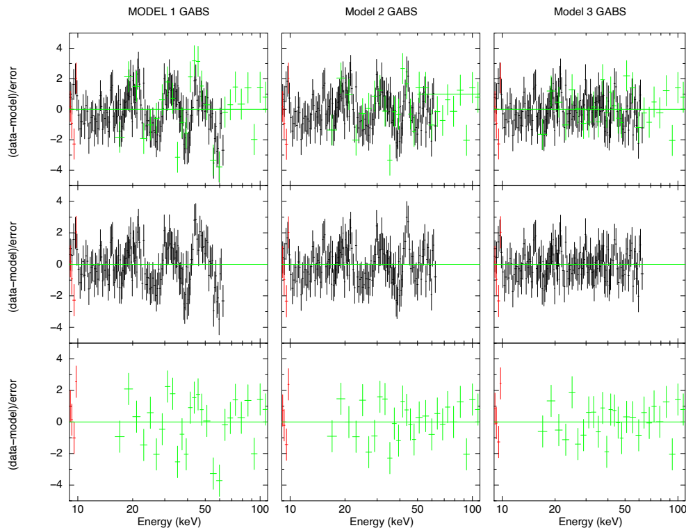
Figure 6. Residuals in units of \sigma for the XRT+FPMAB+BAT data (upper panels), XRT+FPMAB (middle panels), and XRT+BAT (lower panels), using the BWMODEL with one Gaussian absorption line at 38 keV (first column), with two Gaussians at \sim 38 and 61 keV (second column) and with two nested Gaussians at \sim 38 keV and one at 61 keV (third column). FPMAB data in black, BAT data in green, XRT data in red. We show, for clarity's sake, only the 9–110 keV range.
