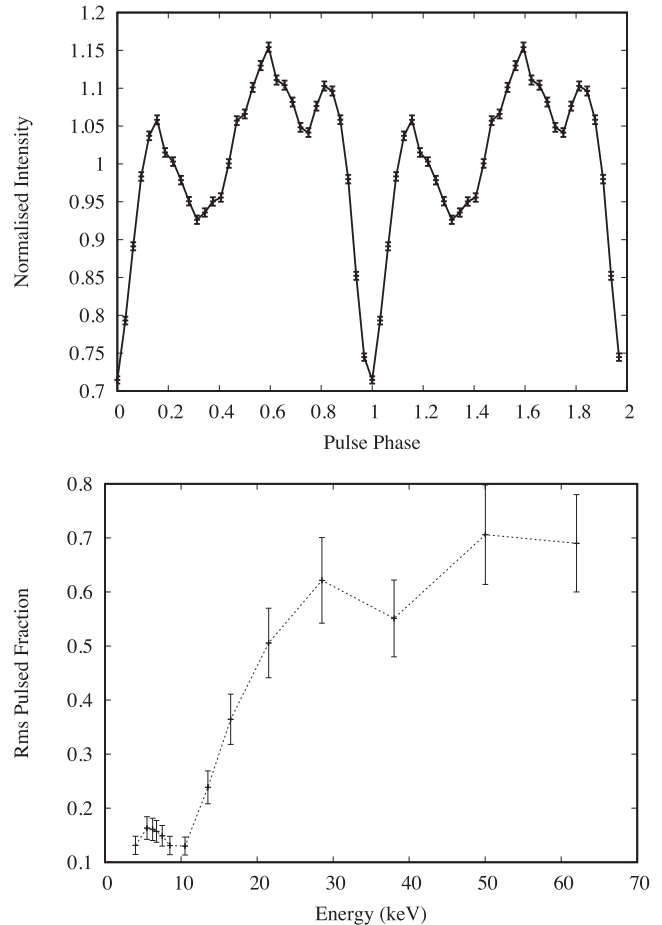
Figure 9. Upper panel: folded profile of the pulsed emission of 4U 1626–67 in the whole NuSTAR band. Lower panel: rms pulsed fraction versus energy.
