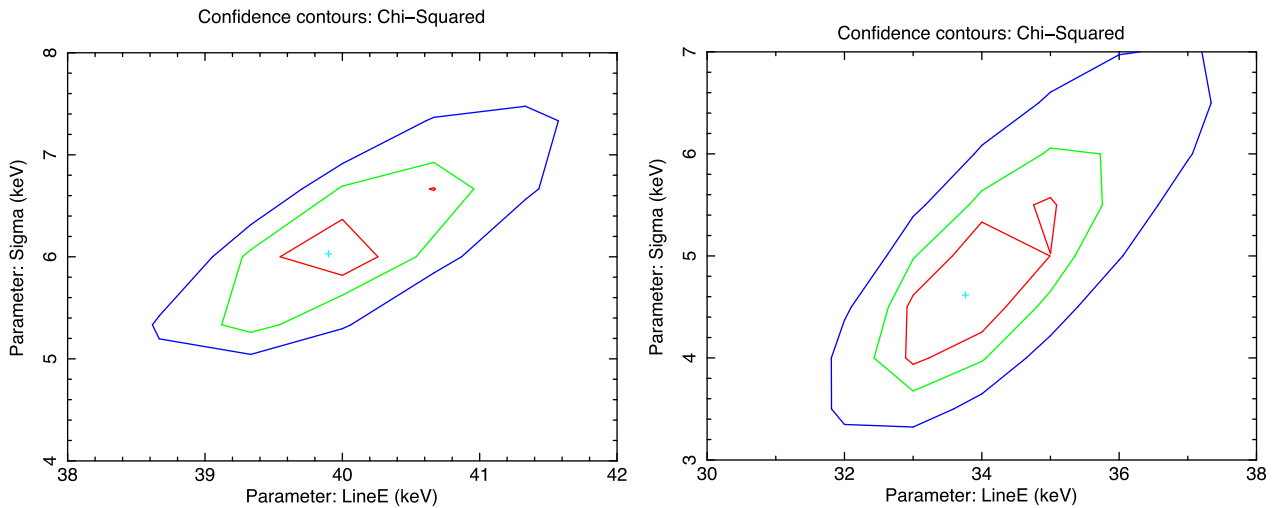
Figure 12. Contour plots for the cyclotron line energy position and width for two phase-selected spectra corresponding to interval 0.2 (left-hand panel) and phase interval 0.0–0.15 (right-hand panel). Confidence intervals at 68 (red contour), 90 (green contour) and 99 per cent (blue contour).
