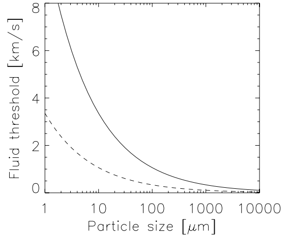
Fig. 19. Fluid threshold velocity calculated using the Shao-Lu formulation with values for gravity appropriate for 67P ( g = 1.55 \times 10^{-4} \text{ m/s}^2 ). The velocity rises rapidly as the particle size decreases because of cohesive forces. Gas pressures of 0.003 Pa (solid line) and 0.03 Pa (dashed line) are shown.
