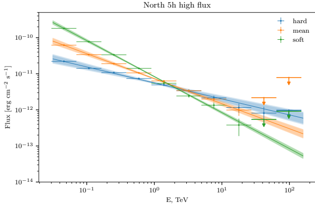
Fig. 4. Simulated spectra of LS I +61° 303 for 5 h observation. The three different spectral slopes are shown. Solid lines represent the power-law spectral fit. The butterfly represents the 1\sigma uncertainty in the fit.
