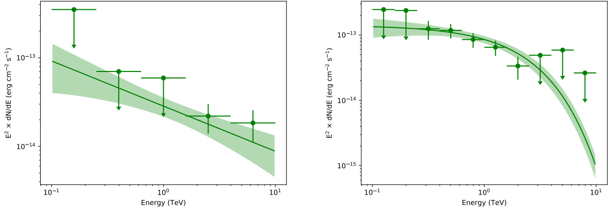
Fig. 15. Simulated spectra of \gamma^2 Vel for extrapolated FL8Y power-law input spectrum ( left ) and for an additional hard component (power law with \Gamma = 2.0 and with E_{\text{cut}} = 2 TeV cut-off, right ). A 50 h observation was used for the simulation.
