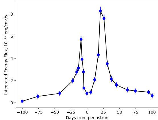
Fig. 3. Simulated light curve above 1 TeV of PSR B1259–63 around periastron. Each point has a 30 min exposure.
