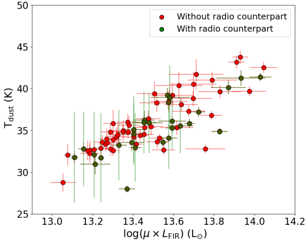
Figure 3. Dust temperatures versus FIR luminosities (uncorrected for magnification) for the 80 (candidate) strongly lensed galaxies from Negrello et al. (2017) . Green and red dots show respectively sources with and without radio counterpart.
