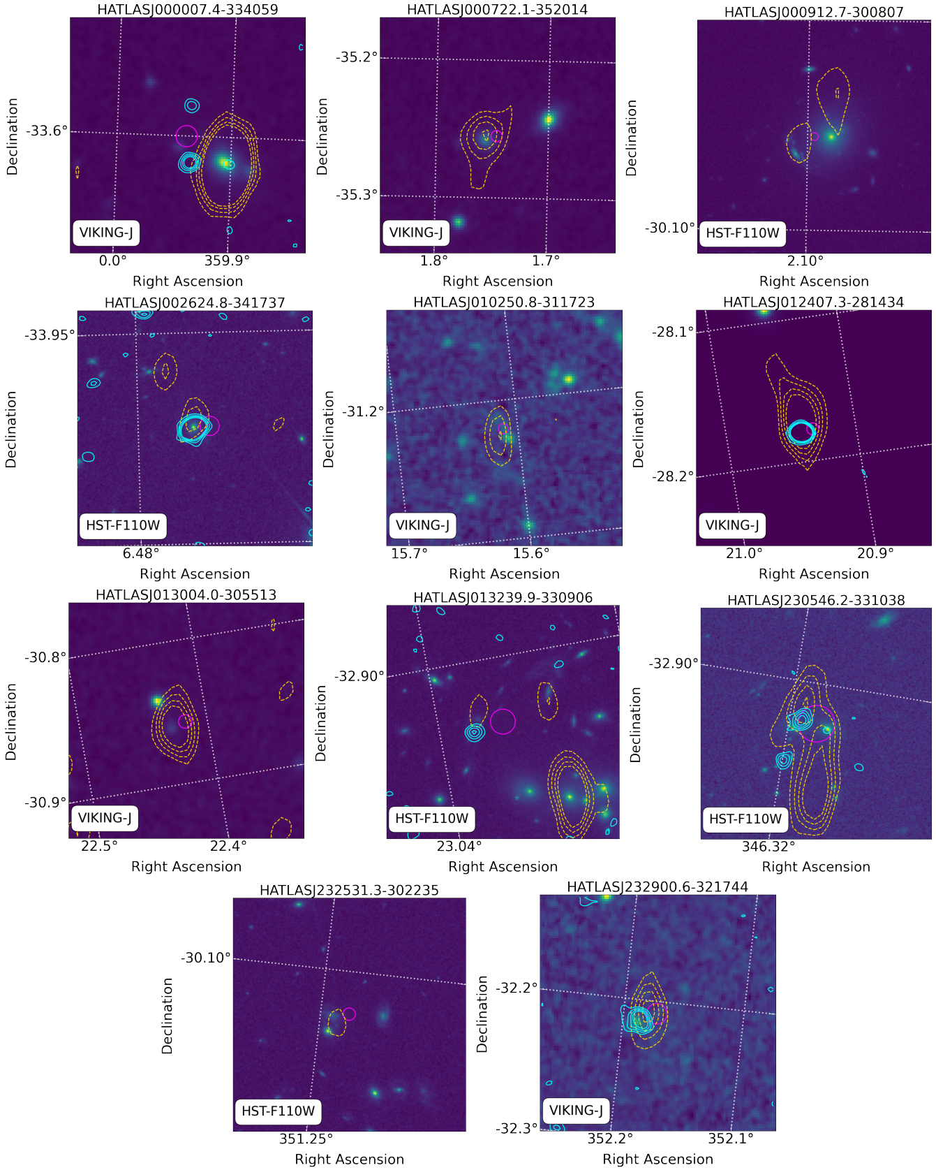
Figure 1. Cutouts of NIR images with the best available angular resolution centred on the Herschel positions for the 11 sources with an ATCA cross-match. Contours at 3,5,7,9 \sigma levels are showed in gold for the radio and cyan for ALMA. Circles are the SPIRE position with a 3\sigma_{\text{pos}} radius. RA and Dec are reported in Deg units. The postage stamps are 30x30 arcsec
