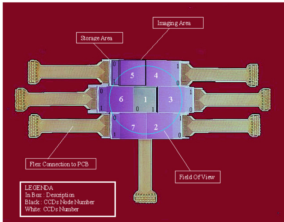
Figure 4.2-3: EPIC MOS Focal Plane
