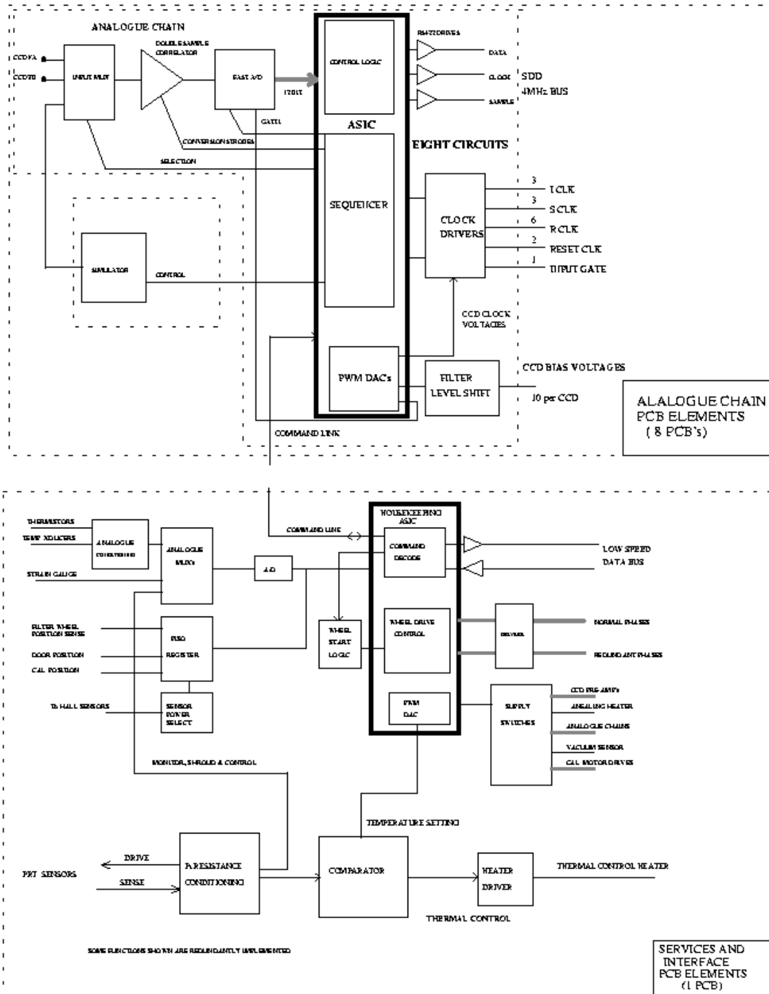
Figure 4.3-1: EMA Block Diagram
