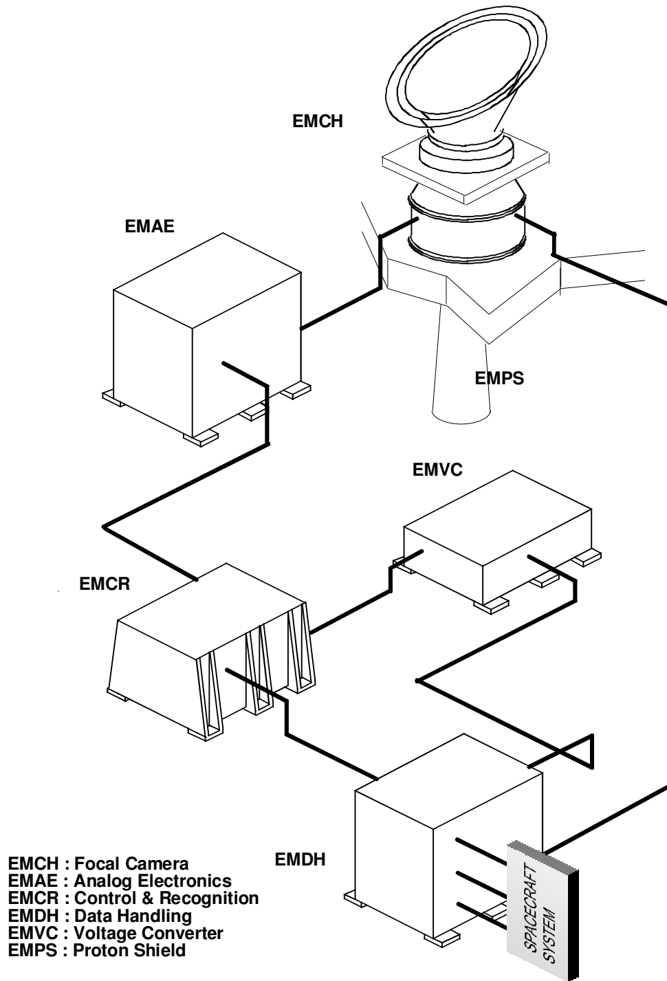
EMCS BLOCK DIAGRAM
