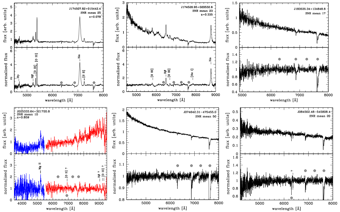
Figure 3. Spectra of three UGSs and three AGUs. Top and lower panels as in Figure 1. Red and blue spectra show the two sides of the dual-beam spectrograph used at Palomar.
