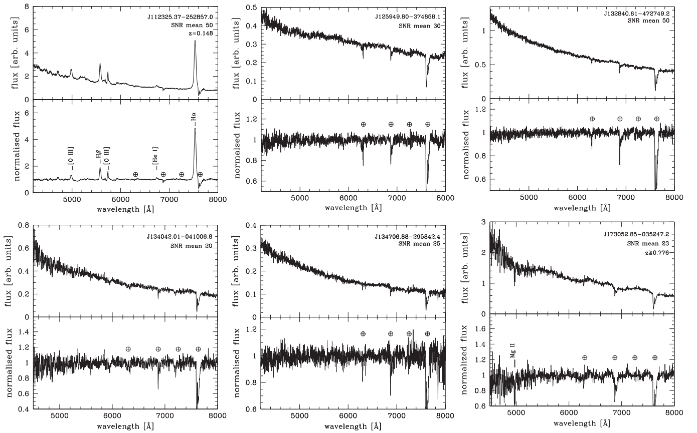
Figure 2. Spectra of six UGSs. Top panels contain WISE name of the potential counterpart, the average S/N and the z when identification of emission and/or absorption lines was possible. Lower panels show the normalized spectrum. The symbol \oplus indicates atmospheric telluric features.
