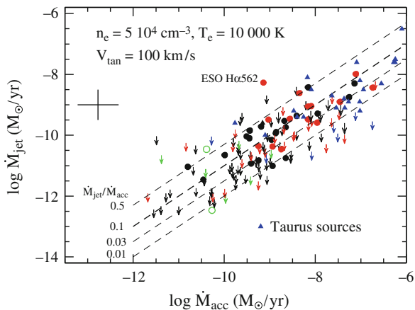
Fig. 3 Mass accretion ( \dot{M}_{acc} ) vs mass ejection ( \dot{M}_{jet} ) rates. The \dot{M}_{jet} has been measured from the [OI]6300Å luminosity assuming a jet tangential velocity of 100 km s ^{-1} and gas temperature and density of 10,000 K and 5 \times 10^4 cm ^{-3} respectively. Black, red and green symbols are as in Fig. 1, while blue triangles indicate the values for the sample of Taurus sources (see text). (From [4])
