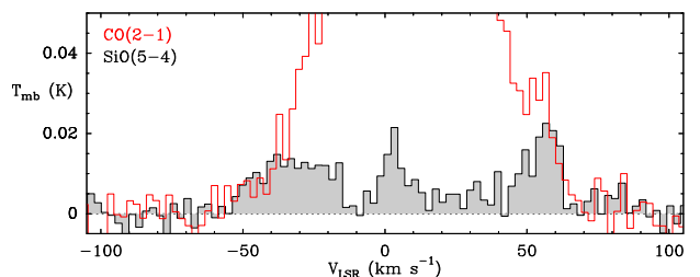
Fig. 6. Spectra of CO(2-1) (red) and SiO(5-4) (gray) toward L1157-mm. Note that the CO(2-1) line, which does not reveal distinct EHV emission, has similar velocity extents as the SiO(5-4) line with the same intensity level.
