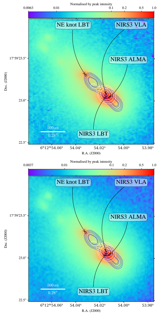
Fig. C.3. Same as Figure 2 but for the filters H 2 (top panel) and Br γ (bottom panel).
