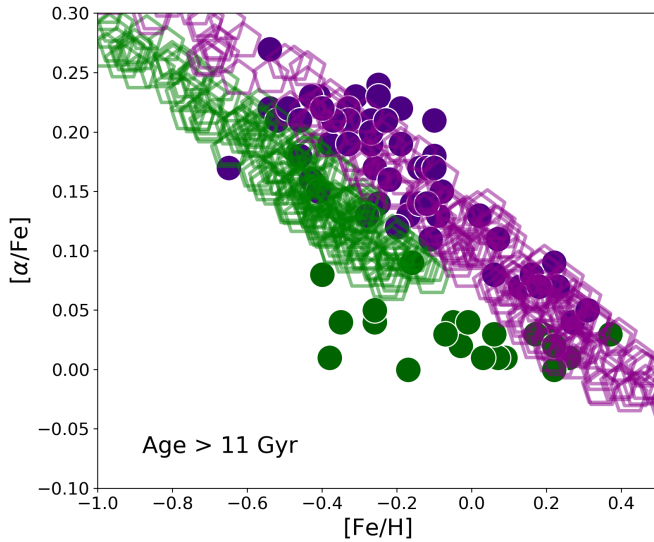
Fig. 20. Abundance ratios of [\alpha/\text{Fe}] as a function of [\text{Fe}/\text{H}] predicted by means of the parallel chemical evolution model including age and [M/H] errors for the high- \alpha and low- \alpha model phases (empty magenta and green pentagons, respectively). Both models and data are related to stars older than 11 Gyr.
