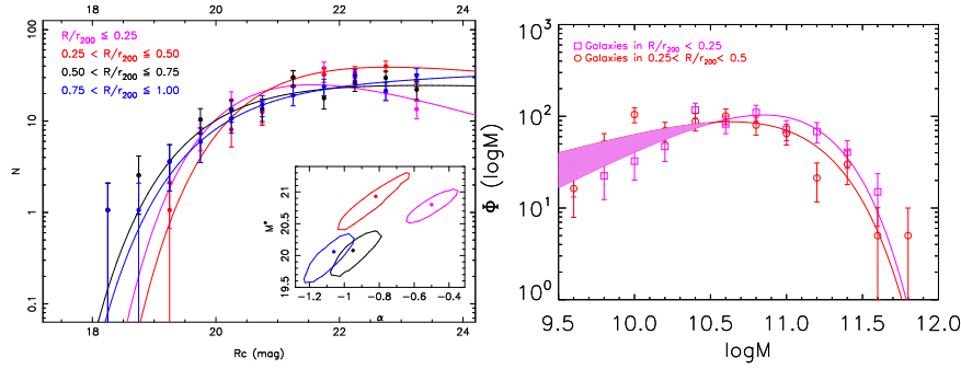
Fig. 1 Left panel : LFs of galaxies in MACS J1206.2-0847, covering regions with increasing distance from the centre. Continuous lines are the fits with the Schechter function. The best-fit Schechter parameters for \alpha and M^* with their 1\sigma contours for the corresponding LFs are also reported in the small panel. Right panel : MFs of galaxies in the core of MACS J1206.2-0847 and the outer adjacent ring. The shaded area highlights the deficit of low mass galaxies in the core, which adds up to \sim 6 \times 10^{11} M_{\odot} (see Annunziatella et al. 2014 for details).
