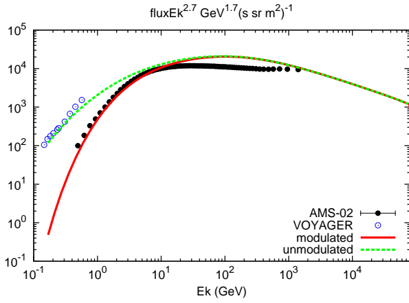
(a) Model-A: CR spectrum.
