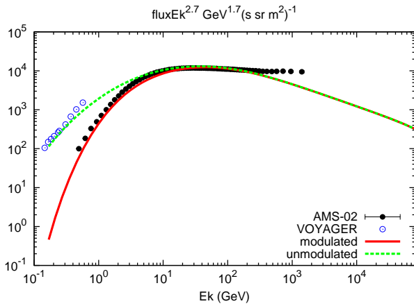
(c) Model-C: CR spectrum.
