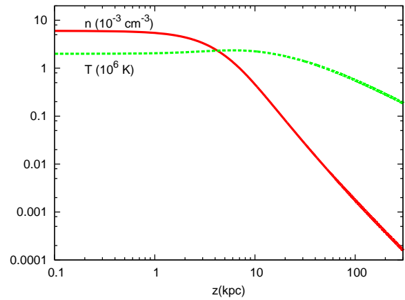
(b) Reference case: gas density and temperature.
