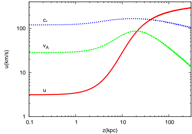
(a) Reference case: velocities.
