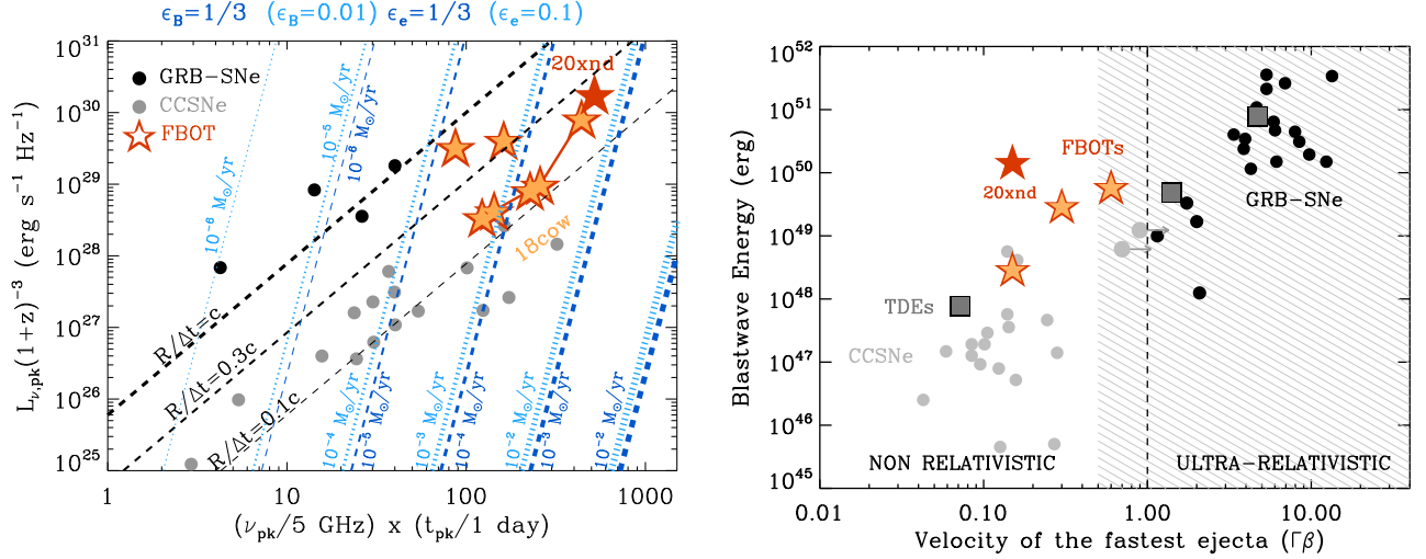
Figure 6. Left Panel: Radio phase-space of stellar explosions, where L_{\nu, \text{pk}} is the spectral peak luminosity, \nu_{\text{pk}} is the spectral peak frequency and t_{\text{pk}} is the peak time. Normal core-collapse stellar explosions (CCSNe, gray filled circles) typically show a shock velocity \sim 0.1c , while GRB-SNe (Black filled circles) are characterized by significantly faster shocks. The new class of multiwavelength FBOTs (stars) is currently comprised of four elements and shows a variety of shock velocities that bridge the gap between normal SNe (e.g., AT2018cow) and the ultra-relativistic jets of GRBs (e.g., CSS 161010, AT2018lug and AT2020xnd). Dashed dark (dotted light) blue lines: lines of constant equivalent mass-loss rate for an assumed wind velocity v_w = 1000 \text{ km s}^{-1} for equipartition parameters \epsilon_B = \epsilon_e = 1/3 ( \epsilon_B = 0.01 , \epsilon_e = 0.1 ). Black dashed lines: lines of constant apparent velocity R/\Delta t under the assumption of equipartition. The factor (1+z)^{-3} accounts for the difference between the angular distance and the luminosity distance. Right Plot: Shock energy vs. fastest ejecta velocity for a variety of transients, including TDEs, SNe and FBOTs. FBOTs represent a new class of transients with energetic shocks that can be transrelativistic. Among FBOTs, AT2020xnd shows the largest equipartition energy. Same color coding as panel on the left. Shaded region: parameter space of engine driven explosions. References: Margutti et al. (2019); Ho et al. (2019c); Coppejans et al. (2020).
