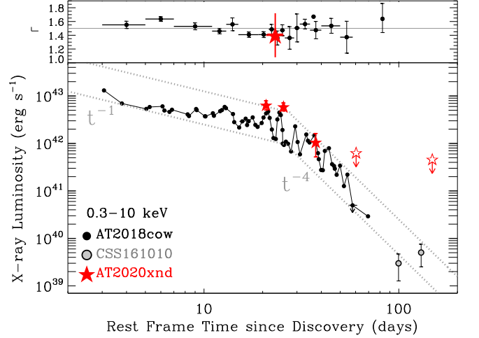
Figure 2. Main Panel: Soft X-ray (0.3–10 keV) luminosity evolution of AT 2020xnd (red stars) compared to the other two known FBOTs with X-ray detections AT 2018cow and CSS161010 (filled black and grey circles, respectively; Margutti et al. 2019; Coppejans et al. 2020). Dotted lines mark a L_x \propto t^{-1} and a L_x \propto t^{-4} power-law decay to guide the eye. Interestingly, AT 2020xnd shows a similar luminosity as AT 2018cow and seems to follow a similar, peculiar temporal evolution, with roughly constant X-ray flux at \delta t \leq 30 d followed by a sharp decay. Upper panel: spectral photon index evolution with time for AT 2018cow and AT 2020xnd. The solid horizontal line is a photon index of 1.5.
