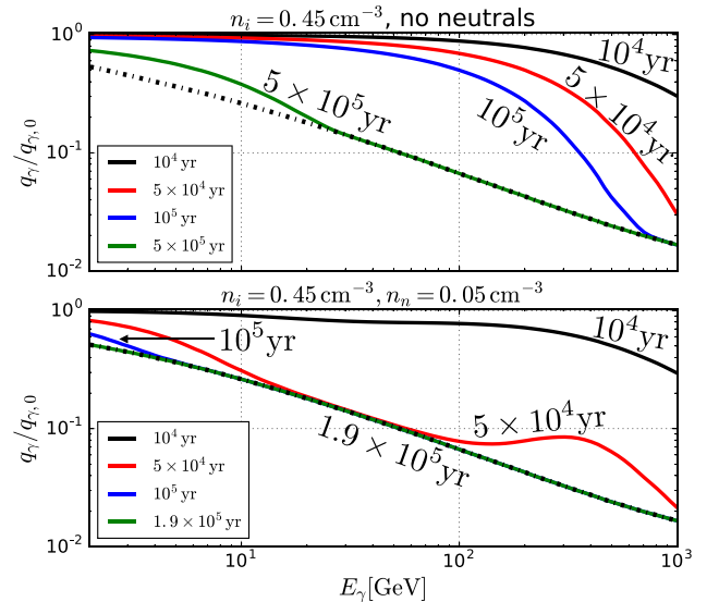
Figure 3. Normalized gamma-ray emission q_\gamma(E_\gamma, t)/q_\gamma(E_\gamma, t=0) (integrated over the flux tube volume) at four different times and for two different types of ISM, as written in the labels. Top panel: fully ionized medium with n_i = 0.45 \text{ cm}^{-3} . Bottom panel: partially ionized medium with n_i = 0.45 \text{ cm}^{-3} and n_n = 0.05 \text{ cm}^{-3} . The black dot–dashed line represents the gamma-ray emission of the Galactic CR pool integrated over the same volume [ f = f_g in equation (20)].
