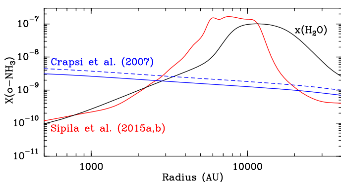
Fig. 3. Radial profile of the fractional abundance of o\text{-NH}_3 with respect to \text{H}_2 , X(o\text{-NH}_3) , in L1544. The blue profile has been deduced from observations carried out by Crapsi et al. (2007) assuming an ortho-to-para \text{NH}_3 abundance ratio of 1 (dashed curve) and 0.7 (solid curve); the red profile is the result of a chemical model calculation by Sipilä et al. (2015a,b). The black profile refers to the total (ortho+para) abundance of \text{H}_2\text{O} from Keto et al. (2014).
