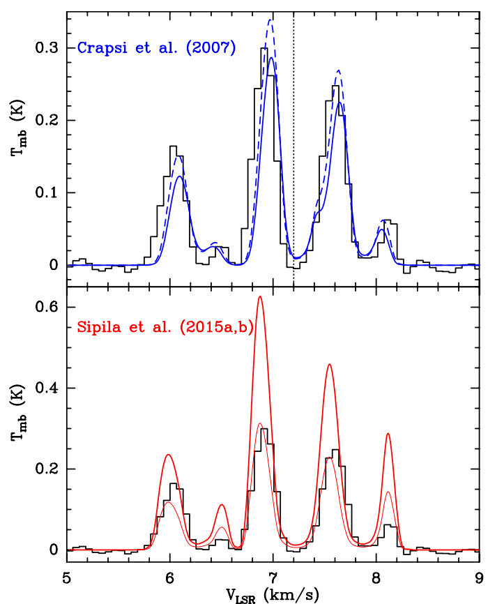
Fig. 4. MOLLIE radiative transfer results using the o\text{-NH}_3 fractional abundance profiles from Fig. 3, overlapped with the observed spectrum: (top) blue solid and dashed curves refer to the Crapsi et al. (2007) profiles, assuming an ortho-to-para \text{NH}_3 ratio of 0.7 and 1.0, respectively. (Bottom) The red thick curve refers to the Sipilä et al. (2015a,b) profile; the red thin curve is the same as the thick red curve, but divided by 2.
