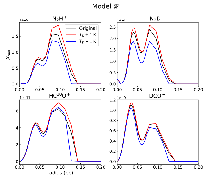
Fig. A.3. Same as Fig. A.1, but for model \mathcal{H} .
