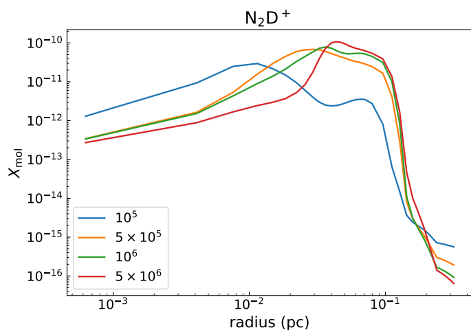
Fig. 7. Abundance profiles for N 2 D + in model \mathcal{L} at four different time steps, from t = 10^5 yr to t = 5 \times 10^6 yr. One can see that as the chemistry evolves, N 2 D + is affected by stronger depletion, with a higher contrast between the central abundance and the peak value.
