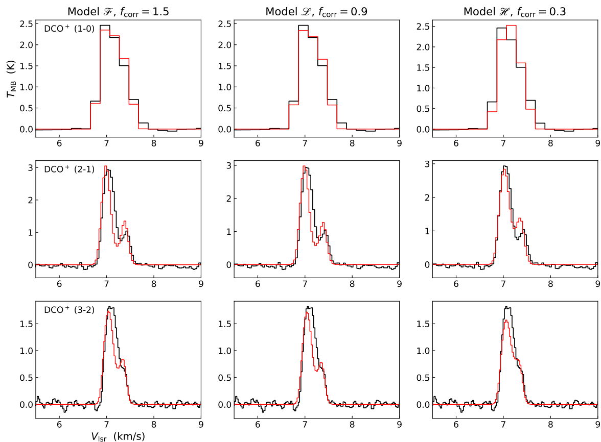
Fig. 6. As Fig. 3, but for DCO + .
