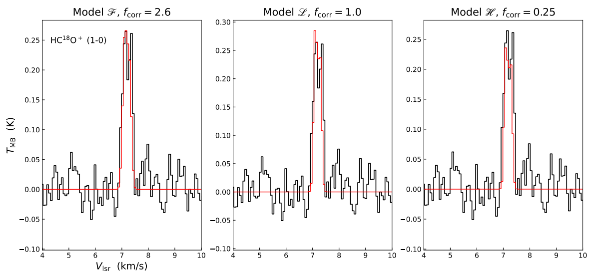
Fig. 5. As Fig. 3, but for \text{HC}^{18}\text{O}^+ .
