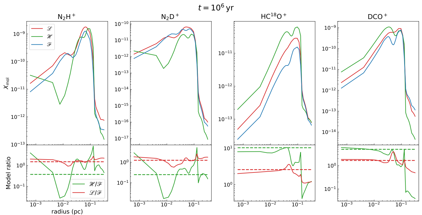
Fig. 2. Top panels: Abundance profiles for the four analysed species (from left to right: \text{N}_2\text{H}^+ , \text{N}_2\text{D}^+ , \text{HC}^{18}\text{O}^+ , \text{DCO}^+ ) at t = 10^6 yr. The colours refer to different models used for the CR ionisation rate: model \mathcal{F} (blue), model \mathcal{L} (red), and model \mathcal{H} (green). Bottom panels: The green and red solid curves show the ratio of model \mathcal{H} and model \mathcal{L} to model \mathcal{F} , respectively. The dashed, horizontal lines represent the inverse ratios of the corrective factors f_{\text{corr}} used to reproduce the observed lines, as reported in Sect. 4.1 and Table 2. To give an example, the radiative transfer of \text{DCO}^+ lines requires f_{\text{corr}} = 0.9 in model \mathcal{L} , and f_{\text{corr}} = 1.5 in model \mathcal{F} ; therefore the red solid curve \mathcal{L}/\mathcal{F} in the rightmost panel has to be compared with the red dashed line at (0.9/1.5)^{-1} = 1.67 .
