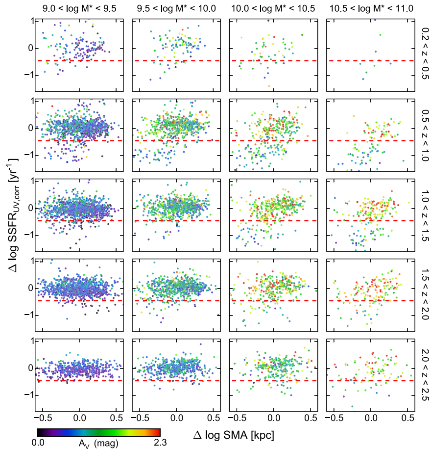
Figure 17. \Delta \log \text{SSFR}_{\text{UV,corr}} vs. \Delta \log \text{SMA} (semimajor axis) for galaxies that lie within the SF region of the UVJ diagram, divided into narrow stellar mass and redshift bins. Points are color-coded by the SED-derived visual attenuation, A_V . Red dashed lines show our criterion to select transition galaxies, \Delta \log \text{SSFR}_{\text{UV,corr}} < -0.45 dex. This value was chosen by eye to best separate ridge line main sequence galaxies from transition objects, which turn out to have low A_V and small radii.
