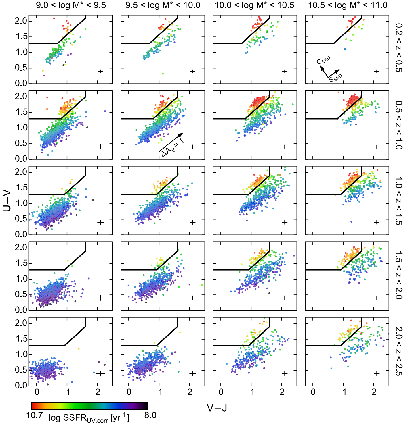
Figure 7. Rest-frame UVJ diagram, divided into narrow stellar mass and redshift bins. Points are color-coded by the dust-corrected, UV-based SSFR, SSFR_{UV,corr} . The arrow is the Calzetti reddening vector for \Delta A_V = 1 mag. The rotated vectors at upper right show the rotated coordinates, C_{SED} and S_{SED} . Crosses indicate the median error bars in U - V and V - J for SF galaxies. The SF sequence shifts to redder colors as age and dust content increase. The quiescent population is seen to form first at higher mass. The shift upwards in U - V (and C_{SED} ) is due to falling SSFRs with time, while the shift to redder V - J is due to more dust. Moreover, a clear gradient in SSFR_{UV,corr} , running nearly parallel to C_{SED} , is seen in all panels except the bottom two with \log M_*/M_\odot < 10.0 and z > 2 .
