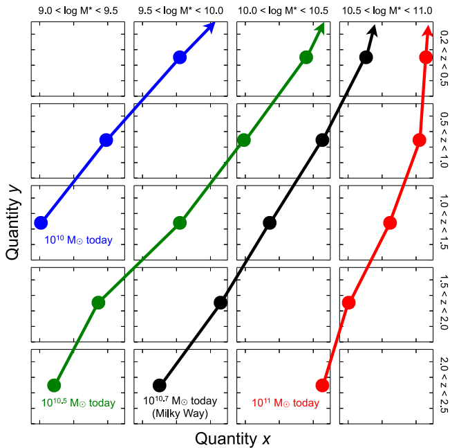
Figure 6. Scatter plots of galaxies in narrow mass and redshift bins arranged in a master grid of mass vs. redshift to illustrate the evolution of galaxy properties. The variables in the scatter plots are arbitrary—they can be UVJ diagrams or any pair of X, Y variables; here they are left empty. Superposed on the scatter plot grid is a separate (and invisible) mass–redshift coordinate system scaled to match the mass–redshift axes of the grid. Mass growth tracks of galaxies are plotted in this separate coordinate system, illustrating how galaxies move through the mass–redshift grid as they evolve. Four representative tracks are shown, labeled by their stellar masses at z = 0 . The vertical positions of the points are the middles of the redshift intervals. The horizontal positions assume that the vertical edges of each panel correspond to the mass limits of each bin. Scatter plots along a given growth track are progenitors and descendants of one another. Galaxies generally evolve diagonally upwards through the grid to higher masses at later times. The Milky Way track is from Papovich et al. (2015), while the others are from Moster et al. (2013).
