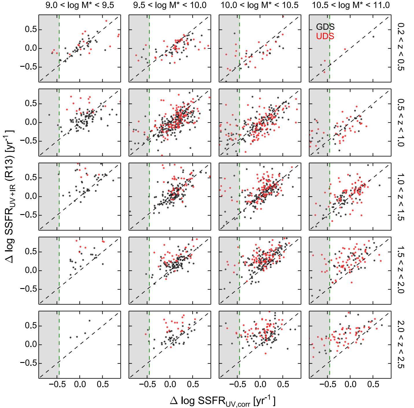
Figure 24. Residuals in \text{SSFR}_{\text{UV+IR}} based on MIPS 24\ \mu\text{m} vs. values of \text{SSFR}_{\text{UV,corr}} from this paper. Residuals are calculated by subtracting the linear fits of \text{SSFR} vs. M_* in Table 2 from both quantities, and so any systematic zero point offset in each panel is preserved. The samples are the same main-sequence ridge line galaxies as in Figures 22 and 23, except that transition galaxies more than -0.45 dex below the fits in Figure 3 are also added (gray regions). Black points are from GOODS-S; red points are from UDS. For SFMS galaxies, systematic offsets of up to \sim 0.2 dex are apparent that vary with redshift. The rms scatter is 0.24 dex, or 0.17 dex if assigned equally to each quantity. In contrast to the main sequence, transition galaxies have systematically high values of \text{SSFR}_{\text{UV+IR}} compared to \text{SSFR}_{\text{UV,corr}} by up to 1 dex.
