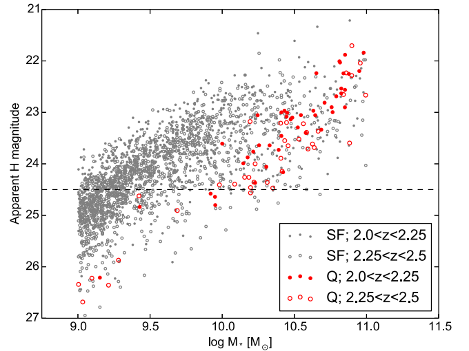
Figure 2. Apparent H magnitude vs. stellar mass M_* in the highest redshift bin z = 2.0-2.5 . The sample magnitude limit at H = 24.5 is shown (dashed line). Quiescent galaxies (which are selected using UVJ ; see Figure 5) are the red points. Filled and open circles are at z = 2.0-2.25 and z = 2.25-2.5 , respectively. SF galaxies are gray. Their vertical width reflects their colors due to dust reddening, with dustier galaxies trending toward fainter H magnitudes. The SF sample at this redshift is strongly biased to bluer galaxies, and dust-reddened galaxies with V - J > 1.2 and M_* < 10^{10} M_{\odot} are largely lost. Nearly all quiescents are captured, except for a handful just below the magnitude limit at 10^{9.5-10} M_{\odot} . (The clump at H \gtrsim 26 is dubious.)
