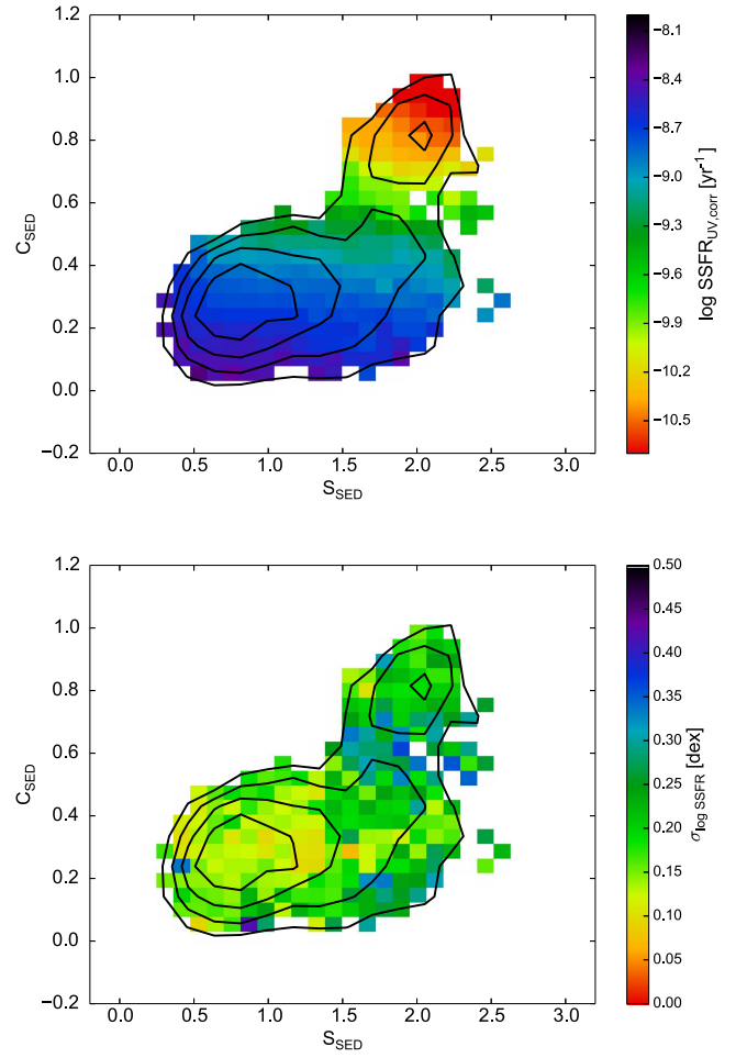
Figure 9. Stacked diagrams using the rotated coordinates C_{\text{SED}} and S_{\text{SED}} . The entire sample is plotted except galaxies with M_* < 10^{10}M_\odot and 2.0 < z < 2.5 (see Figure 8). Black contours are logarithmically spaced and indicate the density of points. The colored 2D pixels show the median value (top panel) and the 1\sigma dispersion (bottom panel) in \log \text{SSFR}_{\text{UV,corr}} in each pixel. Only pixels containing \geq 10 objects are plotted. The top panel shows that \text{SSFR}_{\text{UV,corr}} is correlated with C_{\text{SED}} , while the bottom panel indicates that the typical dispersion in \log \text{SSFR}_{\text{UV,corr}} in a pixel is generally \lesssim 0.25 dex. This small value suggests that the SSFR gradient is a fixed pattern “embedded” in the UVJ diagram, through which galaxies move as they evolve.
