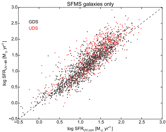
Figure 23. \text{SFR}_{\text{UV+IR}} based on MIPS 24\ \mu\text{m} vs. \text{SFR}_{\text{UV,corr}} from this paper. The samples are the same main-sequence ridge line galaxies as in Figure 22. The black points are from GOODS-S; the red points are from UDS. The dashed line shows equality between the two measures. The total rms scatter of the black points is 0.23 dex; the shallower UDS sample scatters slightly more (0.3 dex).
