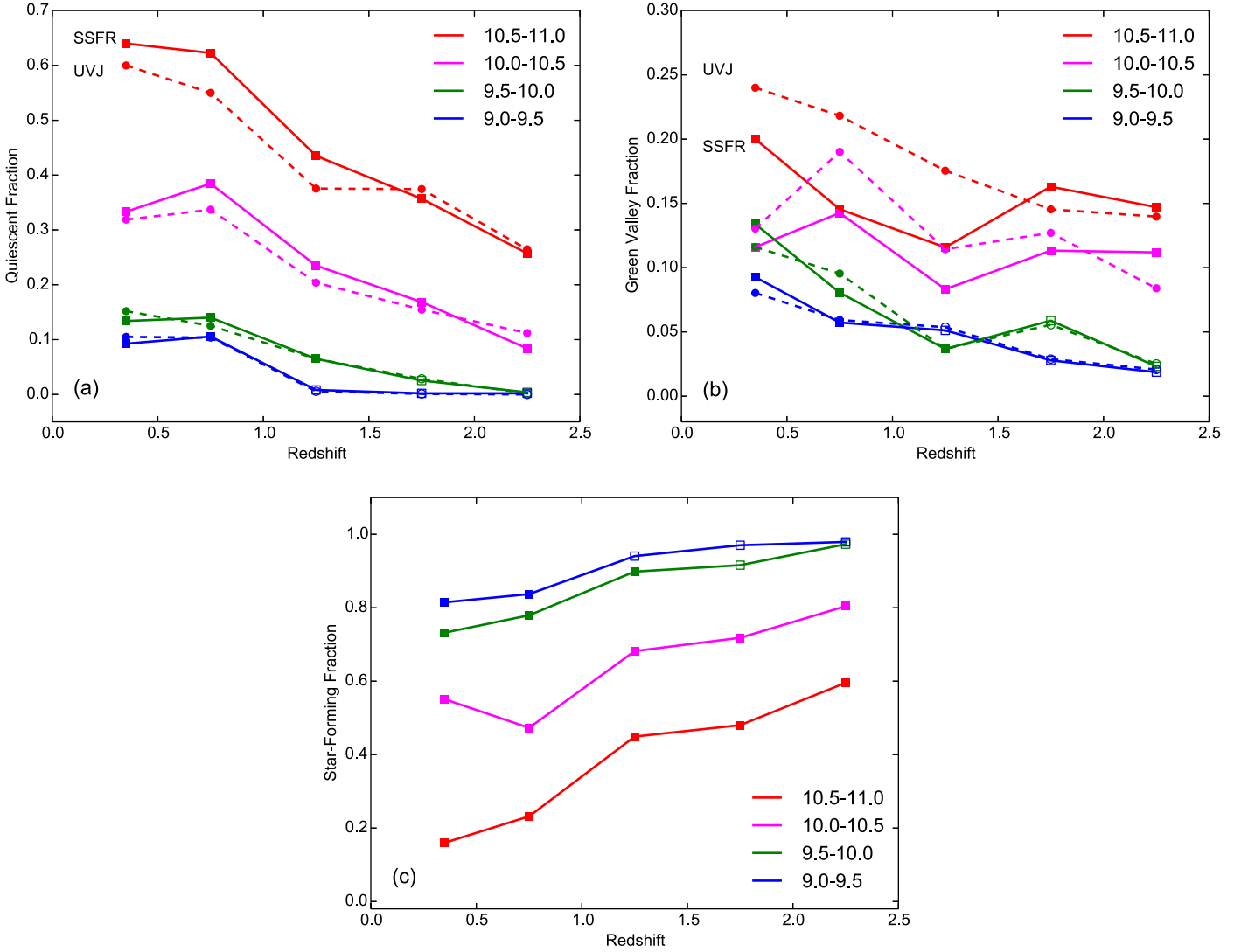
Figure 20. Panel (a): Quiescent fraction as a function of redshift in four stellar mass bins (colored lines). Quiescent galaxies are identified in two ways: \Delta \log \text{SSFR}_{\text{UV,corr}} < -1.0 dex (squares/solid lines) or objects lying within the quiescent region in the UVJ diagram (circles/dashed lines). Panel (b): The green valley fraction, defined as the objects that remain after subtracting off the quiescent and SF galaxies. Panel (c): The SF fraction, defined as the fraction of galaxies with \Delta \log \text{SSFR}_{\text{UV,corr}} > -0.45 dex. In all panels, open symbols denote bins that suffer from incompleteness (the shaded panels in Figure 19).
