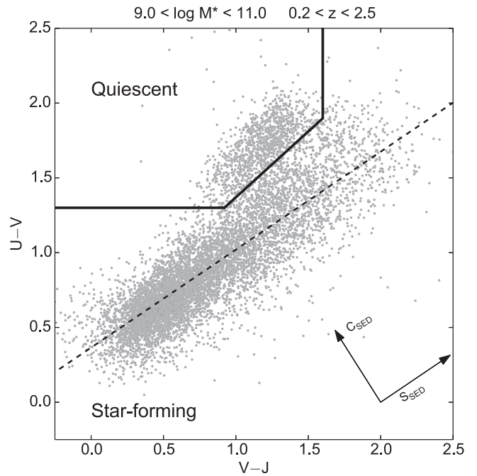
Figure 5. Rest-frame UVJ diagram for all 9135 galaxies in the final sample ( 9.0 < \log M_*/M_\odot < 11.0 and 0.2 < z < 2.5 ). The solid black lines separate quiescent and SF galaxies, according to the definition of Williams et al. (2009) for z = 1-2 . The set of axes in the lower-right corner indicates the rotated coordinates, S_{\text{SED}} and C_{\text{SED}} , that are used to facilitate our analysis. The dashed line indicates the best-fit relation to the SF galaxies used to define S_{\text{SED}} and C_{\text{SED}} .
