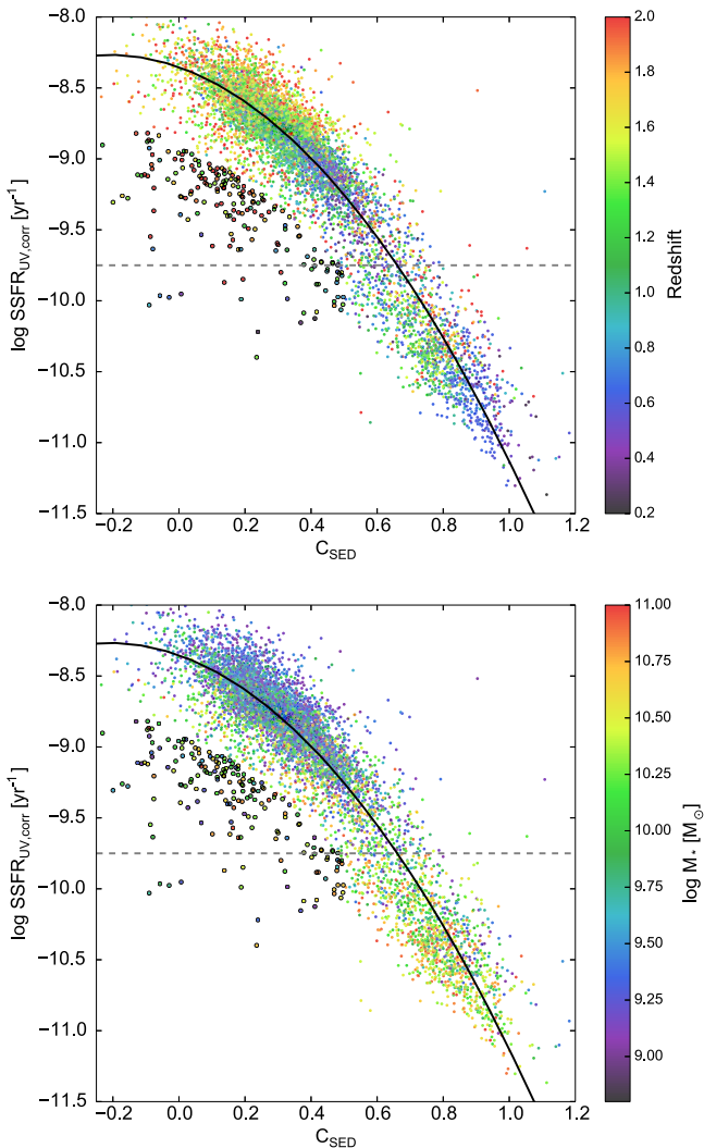
Figure 10. \text{SSFR}_{\text{UV,corr}} vs. C_{\text{SED}} for our sample (excluding objects in the lowest-mass, highest redshift bins, for which C_{\text{SED}} is not reliable; Figure 8). Galaxies are color-coded by redshift (top panel) and stellar mass (bottom panel). The gray dashed line roughly divides the sample into SF and quiescent objects. The black curve indicates the quadratic fit to the data (Equation (6)). The rms scatter in \text{SSFR}_{\text{UV,corr}} about the fit is 0.20 dex (after excluding 2\sigma outliers). Including M_* and z in the fit reduces the scatter to 0.18 dex. Points outlined in black are objects >2\sigma below the relation with C_{\text{SED}} < 0.5 . Most of these aberrant objects turn out to have brighter-than-normal FUV spectra and are discussed further in Sections 3.4 and 4.
