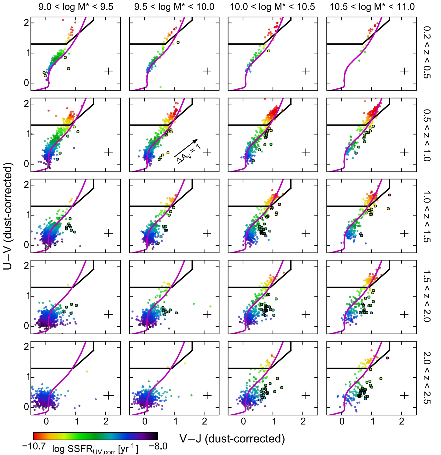
Figure 15. Dust-corrected UVJ diagram, divided into narrow stellar mass and redshift bins. Individual galaxies have been corrected for A_V . Points are color-coded by \text{SSFR}_{\text{UV,corr}} . Error bars represent median uncertainties in the photometry and the derived A_V values. The magenta curve shows the evolutionary track for a dust-free, \tau = 3 Gyr, solar metallicity stellar population model from Bruzual & Charlot (2003). Applying the dust correction shifts points blueward in both colors, resulting in a narrow locus of points that roughly coincides with the stellar population model. Points outlined in black are the bright-FUV aberrant galaxies that lie low in Figure 10. They account for nearly all the points that scatter to the right of the dust-free track, due to their having low returned values of A_V .
