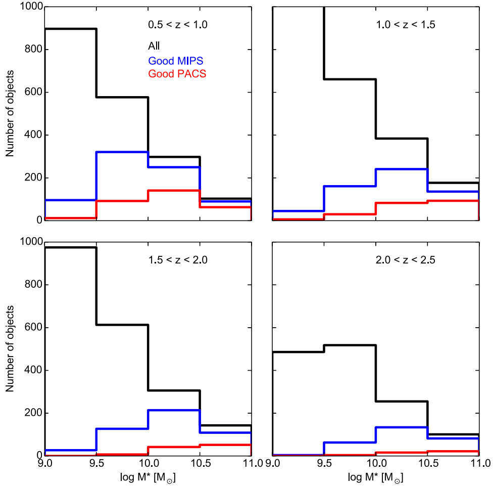
Figure 21. Histograms showing numbers of galaxies in four redshift bins vs. stellar mass. The black histogram (“All”) shows the whole sample of 8060 SF galaxies from Table 1. (This includes transition galaxies as well as SFMS galaxies.) The overlotted blue histogram shows the galaxies in the All sample that have good Spitzer /MIPS 24 \mu\text{m} data, and the overlotted red histogram shows the number of galaxies with good Herschel /PACS data at 100 \mu\text{m} .
