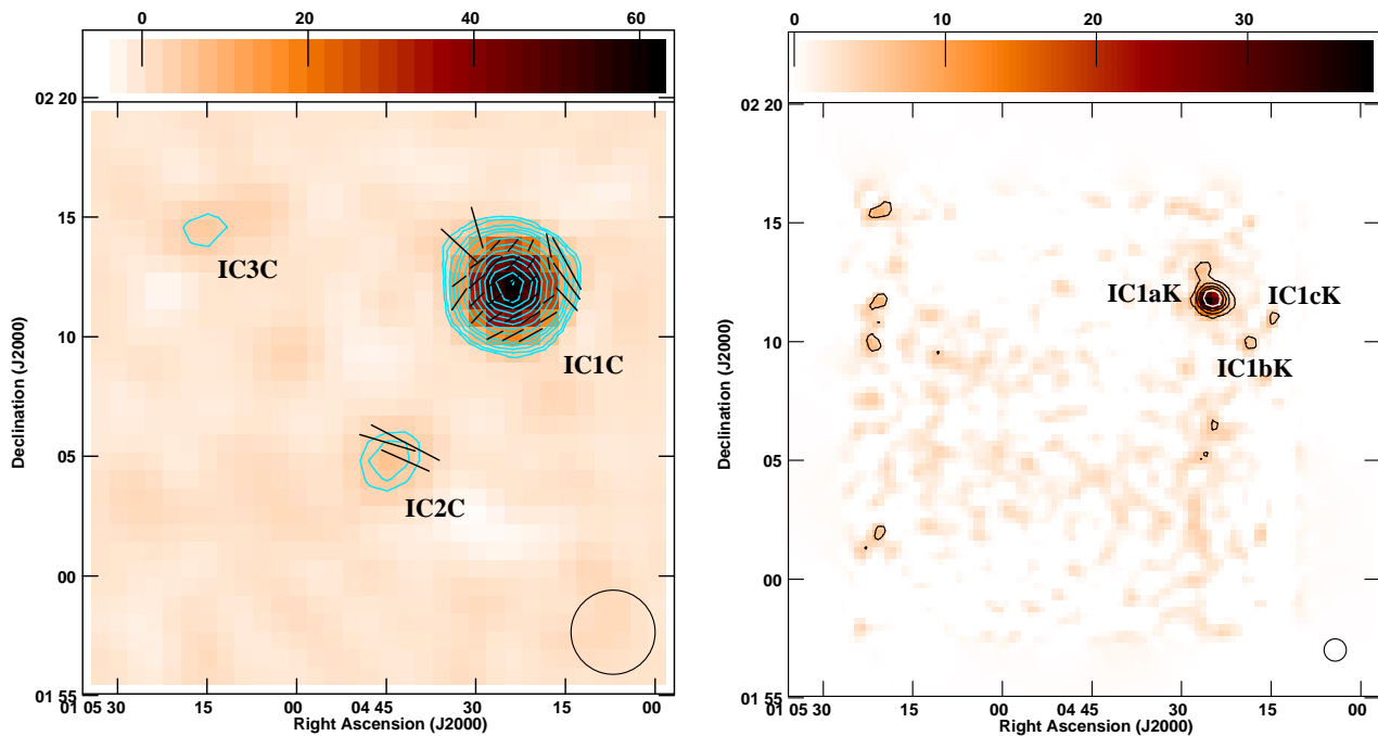
Figure 2. Left: SRT C-band total intensity 21' \times 21' image of IC 1613 resulting from the spectral average of the inner 80% of the bandwidth. The FWHM beam is 2.9 arcmin (bottom-right corner). The noise level is 1.0 mJy/beam. Contour levels are 1.0 \times (3, 4, 6, 8, 10, 15, 20, \dots, 80) mJy. Electric field polarization vectors are overlaid. The length of the vectors is proportional to the polarization percentage (with 10% being a bar of \sim 2.1 arcmin), while their orientation represents the polarization angle. The error on the polarization angle is less than 10^\circ , and the fractional polarization is above 3\sigma_{FPOL} . Right: SRT K-band total intensity 18' \times 18' image of IC 1613 resulting from the spectral average of the inner 80% of the bandwidth. The FWHM beam is 0.9 arcmin (bottom-right corner). The noise level is 1.7 mJy/beam. Contour levels are 1.7 \times (3, 6, 9, 12, 15) mJy.
