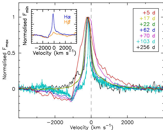
Fig. 3. Selection of continuum-subtracted and peak-normalised H\alpha profiles of SNHunt248. For clarity, only spectra with R > 500 are shown. The inset shows the minimum-normalised +62 d H\alpha and H\beta profiles with identical absorption components. The narrow emission component is resolved only in the +103 d VLT+UVES spectrum.
