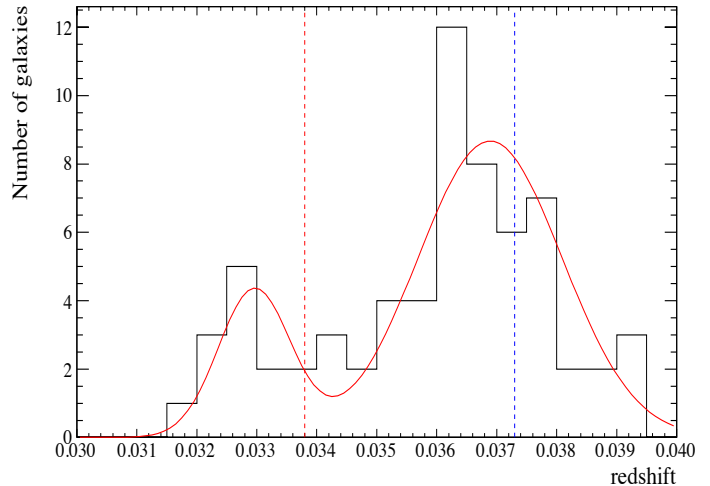
FIG. 8.— Histogram of the redshifts of the final sample of members of Abell 1142 within 1.5 Mpc using a bin size of \Delta z = 0.0005 . Blue and red dashed lines indicate the redshifts of G1 and G2 respectively.
