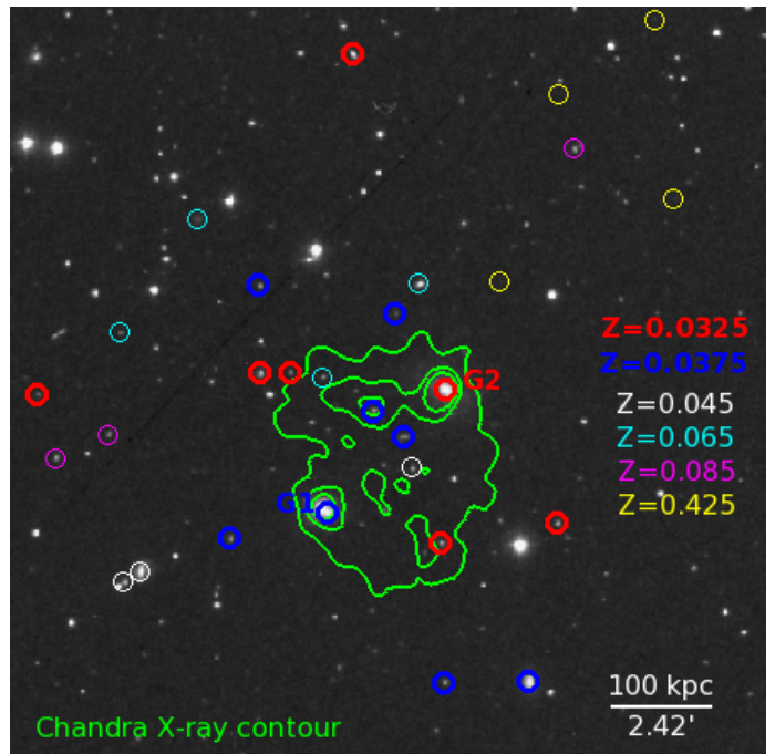
FIG. 5.— . . . DSS image galaxies of the central 18' \times 18' of Abell 1142. Chandra X-ray contour is based on an adaptively smoothed image; contour levels are at [0.9, 1.5, 2.1] \times 10^{-9} photon \text{cm}^{-2} \text{s}^{-1} . We overlaid the redshift distributions of SDSS galaxies (only those with at least three galaxies per redshift bin are shown here).
