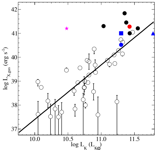
FIG. 11.— Gaseous X-ray luminosities as a function of K -band luminosities for all galaxies taken from Su et al. (2015b). The black solid line is the best-fit L_{X_{\text{gas}}}-L_K relation. Black solid circles indicate group center galaxies. Red circle represents IC664 (G2). Blue symbols represent NGC 3492 (G1)— blue circle: using the average L_{X_{\text{gas}}} and L_K of the three galaxies in G1; blue square: assuming all the L_{X_{\text{gas}}} is from one of the three galaxies; blue triangle: treating all three galaxies as one galaxy (total L_{X_{\text{gas}}} and L_K ). Magenta star represents the small galaxy at the central X-ray peak.
