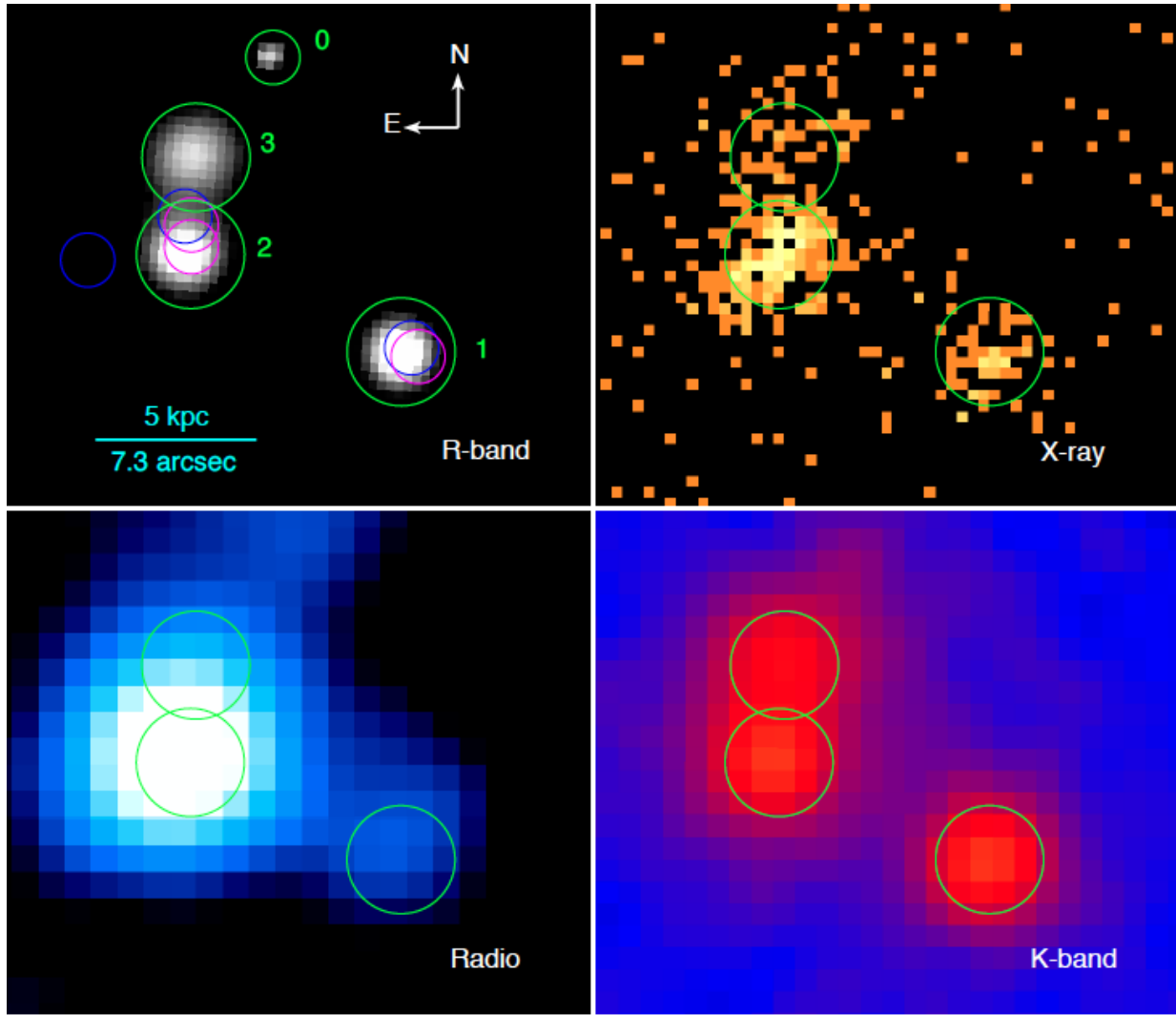
FIG. 9.— . R -band (SDSS), X-ray ( Chandra ), Radio ( VLA ), and K -band (2MASS) images of G1 (NGC 3492) on the same scale. Objects 1, 2, 3 are early-type galaxies. Object 0 is a foreground star. Magenta circles are positions of three galaxies listed in NED and blue circles are three galaxies listed in HyperLeda.
