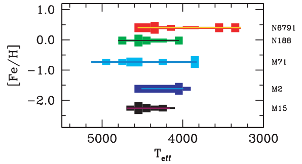
Figure 10. Temperature distribution of red giant stars in each of the five clusters of our sample, according to Tables 11 and 12. Line thickness is proportional to the star density along the spanned temperature range. Note that only cluster NGC 6791 contains stars cooler than \sim 3800 K.
