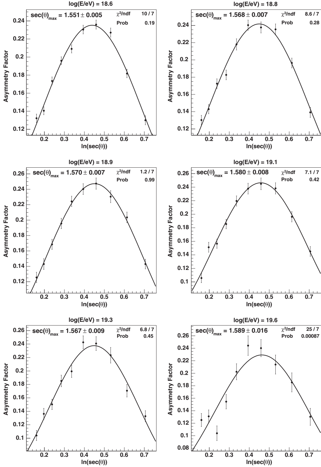
FIG. 6. Asymmetry longitudinal development in bins of \log(E/\text{eV}) at the interval 500–1000 m. From left to right and top to bottom: 18.55–18.70, 18.70–18.85, 18.85–19.00, 19.00–19.20, 19.20–19.50 and above 19.50.
