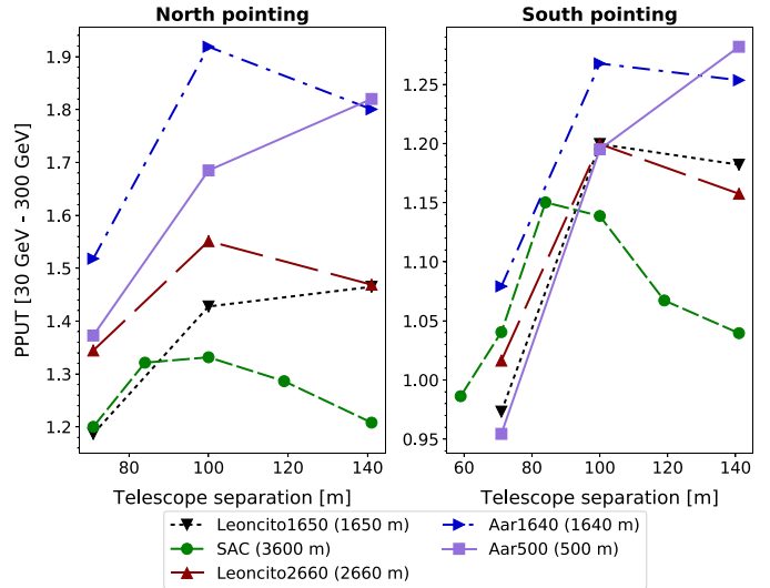
Fig. 7. Performance (expressed in terms of PPUT, see text) of LST squared layouts of different sizes located at different CTA-South candidate sites ( left : Observations towards north, right : Observations towards south), in the energy range 30–300 GeV, using the baseline analysis described in [12].
