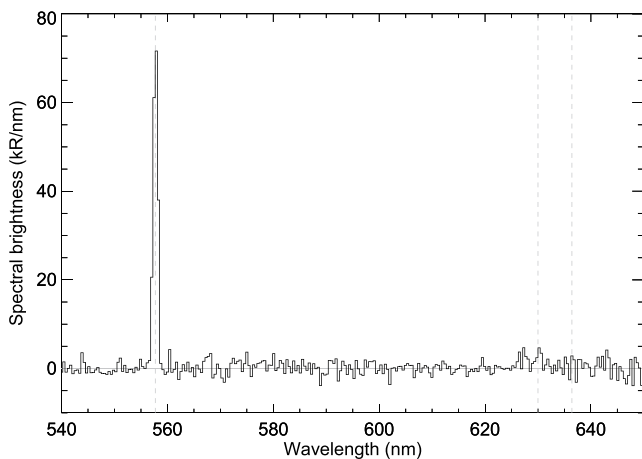
Figure 2. Average visible spectrum from Nadir and Occultation for Mars Discovery/Ultraviolet and Visible Spectrometer spectra obtained from 2531 spectra acquired between 75 and 140 km, for SZA <math><70^\circ</math> and all L_s . Vertical dashed lines represent the predominant oxygen green line at 557.7 nm and the much fainter red line doublet at 630–636.4 nm.
