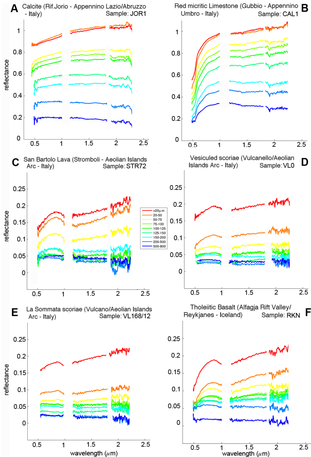
Figure 3. Reflectance spectra acquired with Ma_Miss breadboard setup. The spectra acquired with Ma_Miss BB setup show two gaps in the data at around 1 \mu\text{m} and 1.8 \mu\text{m} , because data are too noisy at the juncture between the Fieldspec 's detectors. See the text for more details.
