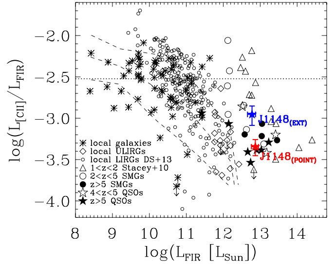
Fig. 13. [C II] /FIR luminosity ratio as a function of FIR luminosity, with our new estimate of L_{[\text{CII}]} / L_{\text{FIR}} in SDSS J1148+5251, obtained separately for the extended and compact components, as explained in Sect. 4.2. For comparison, the plot also includes previous ISO observations of local star-forming galaxies (asterisks, Malhotra et al. 2001) and of local ULIRGs (diamonds, Luhman et al. 2003) along with their median and scatter (dashed lines), recent Herschel /PACS observations of local LIRGs (small open circles, Díaz-Santos et al. 2013), the CSO-ZEUS survey of star forming and active galaxies at redshift 1 < z < 2 (triangles, Stacey et al. 2010), observations of sub-millimetre galaxies (SMGs) at 2 < z < 5 (open circles, Ivison et al. 2010; De Breuck et al. 2014; Valtchanov et al. 2011; Cox et al. 2011; Swinbank et al. 2012; Carniani et al. 2013), sub-millimetre galaxies (SMGs) at z > 5 (filled circles, Riechers et al. 2013, 2014; Neri et al. 2014; Rawle et al. 2014), quasars at 2 < z < 5 (open stars, Maiolino et al. 2009; Wagg et al. 2010; Carniani et al. 2013), and z > 5 quasars (filled stars, Venemans et al. 2012; Wang et al. 2013; Willott et al. 2013). The dotted horizontal line indicates the Milky Way value ( L_{[\text{CII}]} / L_{\text{FIR}} \sim 3 \times 10^{-3} , Carilli & Walter 2013). All measurements refer to the FIR luminosity as integrated over 42.5\text{--}122.5 \mu\text{m} . Where necessary, we have converted L_{\text{FIR}(40\text{--}500 \mu\text{m})} and L_{\text{TIR}(8\text{--}1000 \mu\text{m})} into L_{\text{FIR}(42.5\text{--}122.5 \mu\text{m})} by using the conversion factors provided by Carilli & Walter (2013), i.e. L_{\text{FIR}(40\text{--}500 \mu\text{m})} \simeq 1.2 L_{\text{FIR}(42.5\text{--}122.5 \mu\text{m})} and L_{\text{TIR}(8\text{--}1000 \mu\text{m})} \simeq 1.3 L_{\text{FIR}(40\text{--}500 \mu\text{m})} .
