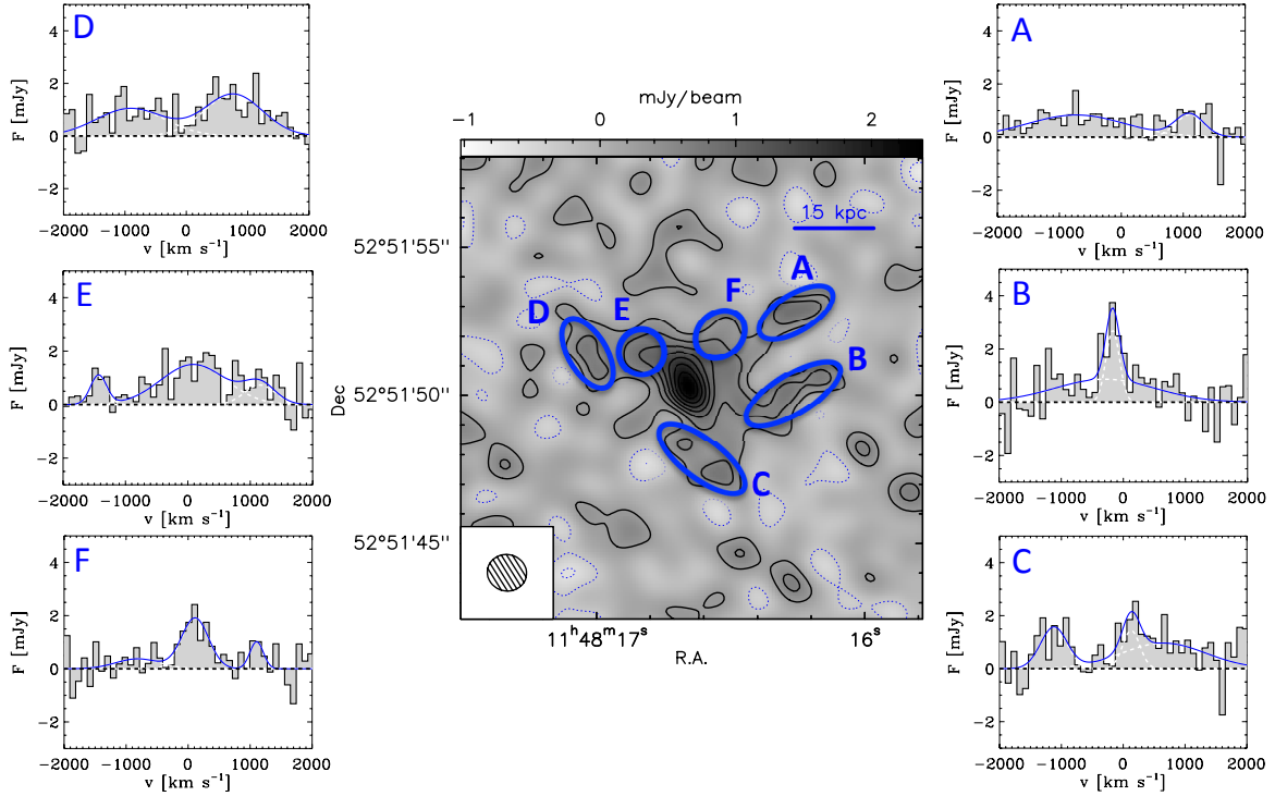
Fig. 3. IRAM PdBI continuum-subtracted map of the total [C II] 158 \mu\text{m} emission of SDSS J1148+5251, integrated within v \in (-1400, 1200) \text{km s}^{-1} , along with spectra extracted from different positions on the source. Negative and positive contours are in steps of 3\sigma ( 1\sigma rms noise is 0.26 \text{ Jy beam}^{-1} \text{ km s}^{-1} ). For display purposes, the spectra have been re-binned by a factor of 4, corresponding to channels of 93.6 \text{ km s}^{-1} . The Gaussian fits to the line profiles are performed on the original non-binned spectra and the fits results are presented in Table B.1.
