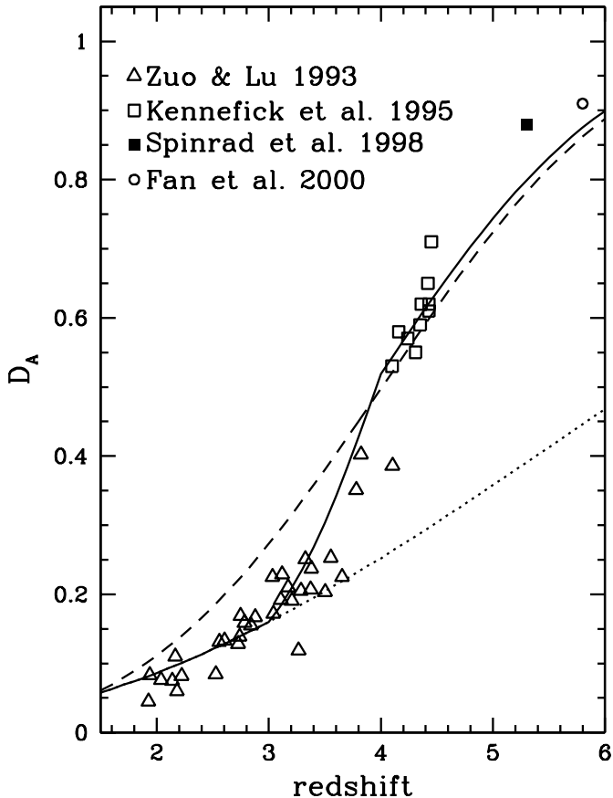
Fig. 2. The deficit D_A in quasars fluxes due to the accumulated absorption of the Ly \alpha forest. The dashed line is obtained by describing the IGM opacity according to the prescriptions by Madau (1995), while the dotted line are those by Scott et al. (2000). The solid line is the model adopted in this paper. References for the data points are indicated. The small difference between the Madau values of D_A and ours at z > 4 is due to the contribution of Ly limit systems (Madau 1995, Eq. (13)), which was not included in Madau’s formulation.
