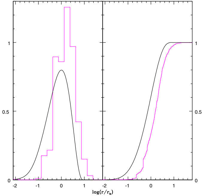
Fig. 1. Left panels: distribution of mass as a function of radius (expressed in half-light radius units) for our sample clusters (black) and distribution of stars observed in this study (magenta). Right panels: cumulative distribution for the mass of our sample GCs (black) and of the stars observed in this study (magenta).
