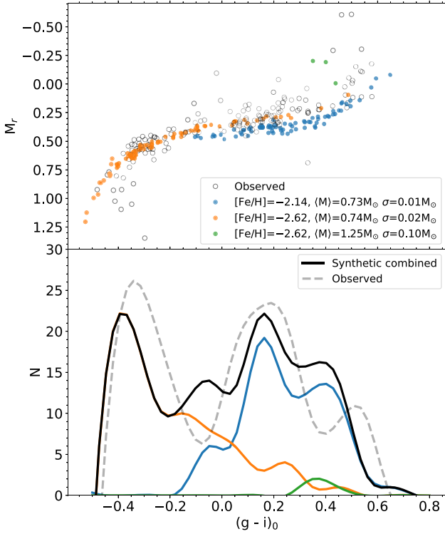
Figure 11. Top: Absolute CMD ( M_r , (g - i)_0 ) for the observed and the simulated HB of Eri II. The constraints for each synthetic populations are labeled in the legend. Bottom: Colour (g - i)_0 distribution of each synthetic population, the synthetic combined, and the observed HB population. The synthetic HB accounts for photometric errors based on Monte Carlo simulations.
