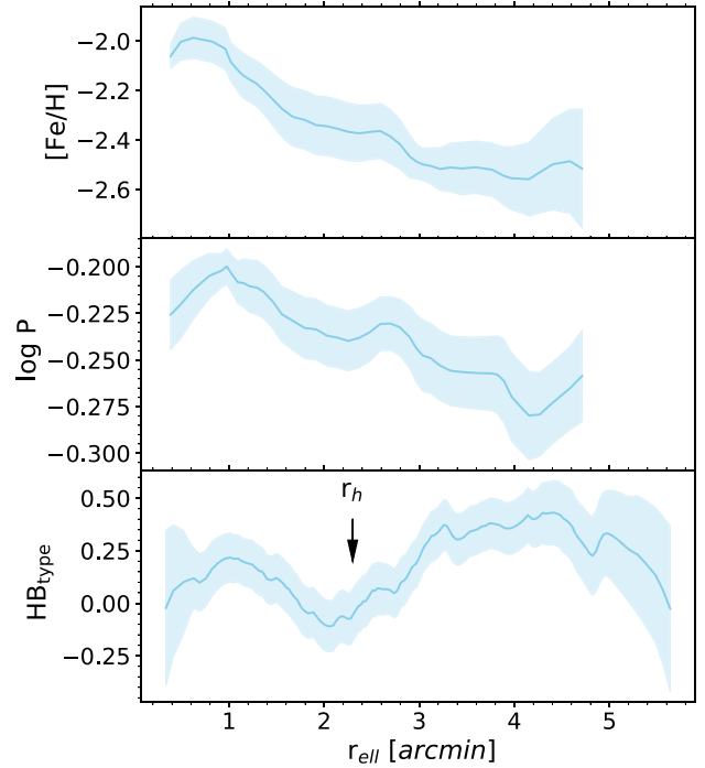
Figure 13. Radial gradient of the metallicity (top), the logarithm of the period (middle), fundamentalized for the RRc types, of the RRL stars in Eri II, and the morphology of the HB ( HB_{\text{type}} , bottom). The blue shaded areas show the corresponding uncertainties.
