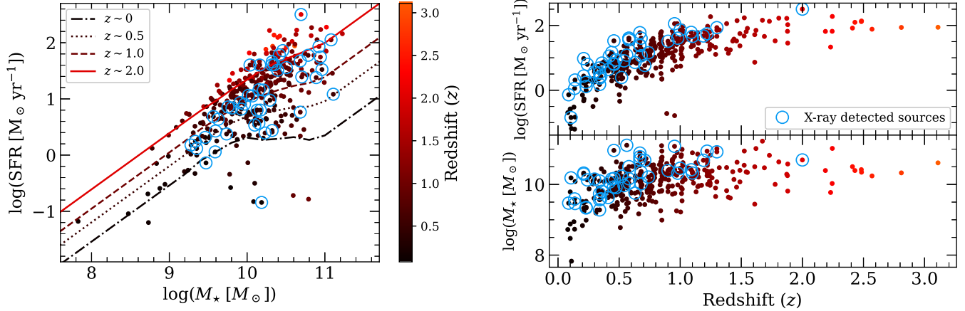
Figure 3. Left: SFR versus stellar mass ( M_* ) for our final sample of 344 galaxies. The four overlaid curves indicate the locations of the galaxy main-sequence for various redshifts that span our sample: z \sim 0 , z \sim 0.5 , z \sim 1.0 , and z \sim 2.0 in the dot-dashed, dotted, dashed, and solid lines, respectively (Whitaker et al. 2014). The data points and main-sequence curves have been colored by redshift for comparison (see color bar). The blue circled points indicate galaxies that were detected in the X-ray (see Section 3.2). Right: SFR and stellar mass ( M_* ) versus redshift for our final sample. Similar to the left, the blue circled points are galaxies that were detected in the X-ray (see Section 3.2), which tend to be relatively nearby and of high SFR and M_* .
