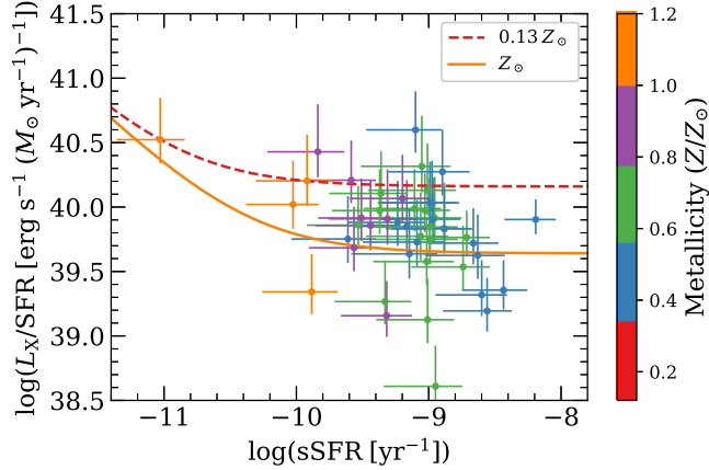
Figure 4. Logarithm of the 2–10 keV luminosity per SFR ( \log L_X/SFR ) versus specific SFR (sSFR) for X-ray detected sources in our sample. The X-ray detected sources (circles with 1\sigma error bars) are compared to local scaling relations, including the L_X/M_* relation for LMXBs from Lehmer et al. (2019) and the metallicity-dependent L_X/SFR relation for HMXBs from Lehmer et al. (2021). Two different relationships are shown corresponding to metallicity values of 0.13 Z_\odot (dashed) and Z_\odot (solid). The detected galaxies largely fall in between the Z_\odot and 0.13 Z_\odot metallicities, which is consistent with the expected metallicity of galaxies in the CDFs.
