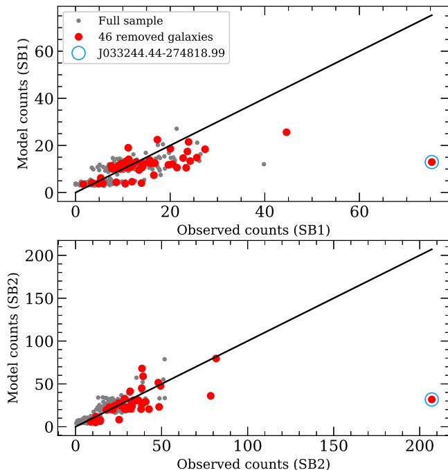
Figure 13. A comparison of model counts versus observed counts in each of the SB1 ( upper ) and SB2 ( lower ). The 344 galaxies of the full sample are shown as small gray points with the 46 removed galaxies (for possibly being undetected AGN, see Section 2) are shown as red points. A one-to-one black line is shown to display where points would lie when the model and observed counts agree. One significant outlier source (J033244.44-274818.99) is highlighted with a light blue circle.
