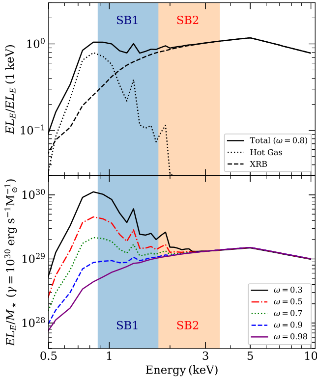
Figure 6. Top: A decomposition of the spectral model used in this study, showing the hot gas and XRB model components as dotted and dashed lines respectively, with the total model spectrum shown as a solid line. The displayed spectrum demonstrates the spectral shape of \omega = 0.8 , similar to the value found for the semi-independent model in Section 4.2. Bottom: The variation of model SED shape as a function of \omega (the fraction of the total 0.5–8 keV luminosity from the XRB model component). These spectra adopt a fixed value of \gamma = 10^{30} \text{ erg s}^{-1} M_{\odot}^{-1} , the 2–10 keV luminosity per stellar mass, and therefore primarily show variations in the hot gas contribution. In both top and bottom panels, the blue and orange shaded regions show the SB1 and SB2 rest-frame energy ranges for z = 0.76 , the median redshift of our sample.
