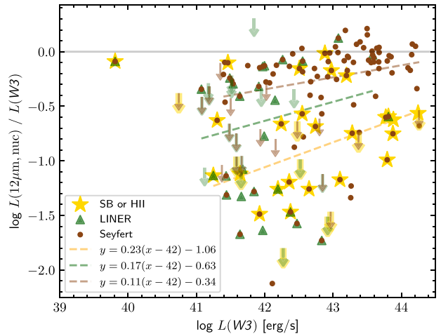
Figure 12. Logarithmic ratio of nuclear 12\mu m luminosity, L^{nuc}(12\mu m) from Asmus et al. (2014) to profile-fitting W3 luminosity, L(W3) , over L(W3) for all 146 objects in common. Objects that are identified as star-forming in the literature (SB or HII) are marked with golden stars, while such with LINER classification have green triangle, and those with Seyfert classifications have brown dots. Objects can have several of these classifications in which cases the corresponding symbols are overlapped. Nuclear 12\mu m non-detections are marked by arrows of the corresponding colours. The light grey line marks the zero line, while the dashed lines provide linear fits to various sub-populations of detections, namely the dark-grey line for all objects only classified as Seyferts, the green line for Seyferts that also have LINER classification but not star-forming and in orange for all objects without Seyfert classification.
