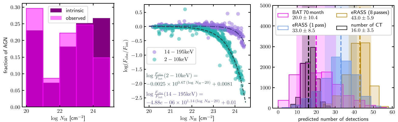
Figure 19. Left-hand panel: normalized distributions of obscuring column density, N_{\text{H}} , for the BAT 70 month AGN sample. In light magenta is shown the observed distribution for the B70 AGN in LASr fulfilling R90, while in dark purple is shown the inferred intrinsic distribution from Ricci et al. (2015). Middle: empirical X-ray extinction curves for the BAT 70 month AGN sample with 10^{20} \leq \log(N_{\text{H}} \text{ cm}^{-2}) \leq 24.5 for observed and intrinsic fluxes as well as N_{\text{H}} values taken from Ricci et al. (2017). In purple is shown the observed to intrinsic flux ratio for the 14–195 keV energy range, while in green the same is shown for the 2–10 keV range. The darker coloured dot-dashed and dashed lines give exponential fits to the data, respectively, with the corresponding best parameters shown as well in the same colour. Right-hand panel: simulated detection rates for Swift /BAT after 70 months (magenta) and SRG /eROSITA after one (blue) and eight all-sky passes (gold). The distributions show the results of the iterations of the Monte Carlo simulation using the intrinsic N_{\text{H}} distribution, while the dashed lines give the median and the shaded areas the standard deviation. These values are given in the legend as well. In addition, the expected number of CT AGN is shown in black.
