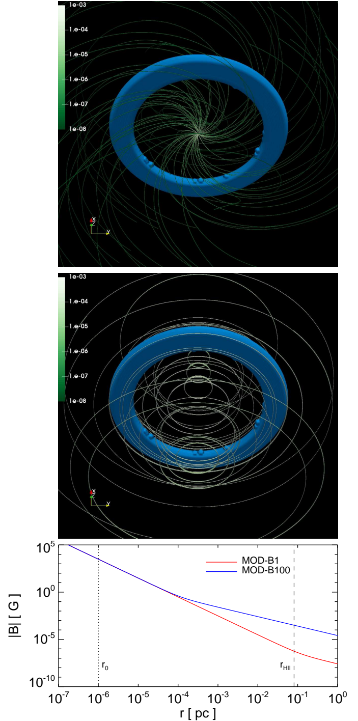
Fig. 1. Initial configuration of the pre-SN ambient magnetic field for models MOD-B1 ( upper panel ) and MOD-B100 ( middle panel ). The green lines are sampled magnetic field lines; the scale of the magnetic field strength is log, shown by the bar on the left of each panel, in units of G. The unshocked equatorial ring material (with n \geq 1000 \text{ cm}^{-3} ) is in blue; the figure does not show the H II region around the ring. Lower panel : radial magnetic field strength in the equatorial plane for the two models; the dotted line indicates the radius of the BSG progenitor, the dashed line the inner edge of the H II region.
