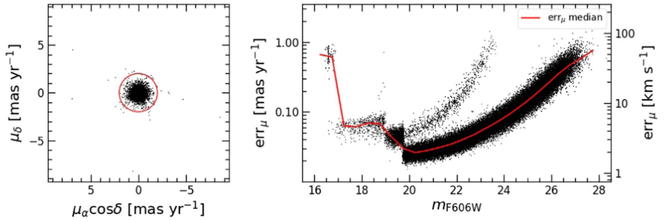
Figure 3. Left panel: VPD of the stars satisfying criteria (i)–(vii), see the text for details. The red circle corresponds to 2 \text{ mas yr}^{-1} , marking the threshold adopted to reject non-cluster members (note, however, the very low level of field contamination). Right panel: 1D PM error as a function of the F606W magnitude for the stars satisfying criteria (i)–(vii). The multiple sequences and discontinuities are due to the different temporal baselines and number of images used to compute the PMs in our project. The red line is the median value of \text{err}_\mu , measured in magnitude bins 0.5 \text{ mag} wide.
